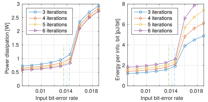
Fig. 10. Power and energy dissipation as a function of input BER for a 7-bl t=3 staircase decoder. Note the order of the curves. The dashed lines show the approximate threshold range for the considered decoder configurations.
