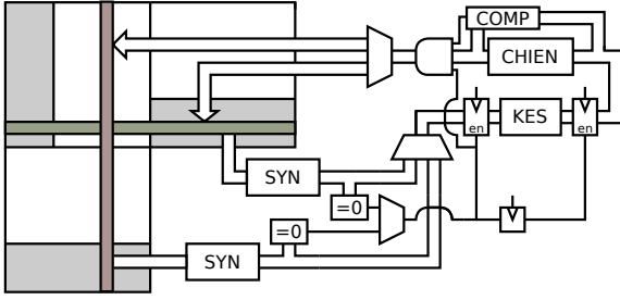
Fig. 2. A 3-block staircase memory array supported by component decoders.
