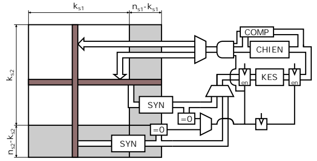
Fig. 1. BCH component decoders used in a product-decoder architecture.
