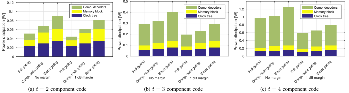
Fig. 5. Power dissipation of the 33%-OH decoders at the 10^{-15} threshold and at a 1-dB margin. Note the dramatically varying scales of the y-axes.
