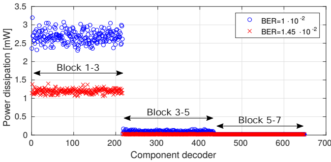
Fig. 9. Power dissipation of component decoder back-ends (KES+Chien) as a function of spatial placement in a staircase window and input BER.
