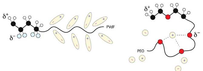
Fig. 7. Schematic illustration of the polymer-ion interactions established in PVdF-HFP (left) and PEO (right) based membranes, the latter being able to promote cation-anion dissociation through favorable O^- – cation interactions. The atoms are coloured as follows: red (O), blue (F), white (H) and black (C).
