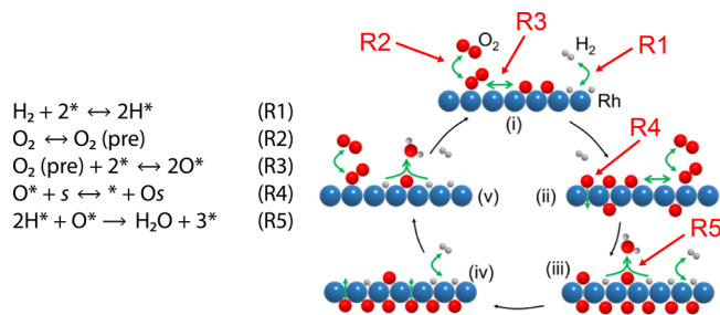
Figure 10. Reaction equations and schematic representation of the reaction steps in H_2 oxidation on Rh. Color code: Rh (blue), O (red), and H (gray). In R1–R5, * and s correspond to empty surface and subsurface sites, respectively.
