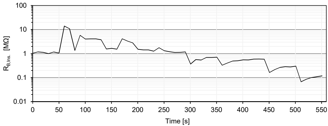
Figure 58. Bearing resistance in insulating state, R_{B,Ins} . (in M\Omega ) of bearing type 22220 at different operating points. R_{B,Ins} . is plotted on a log scale to indicate its subtle changes with respect to speed.
