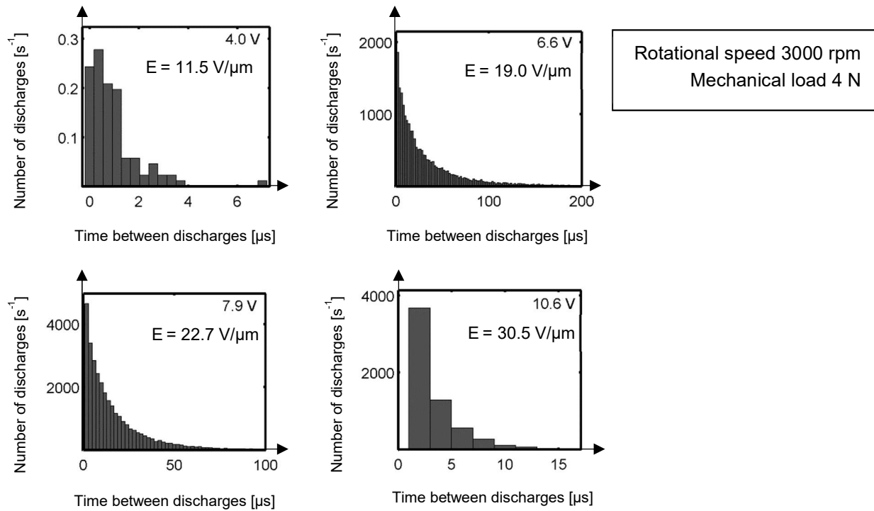
Figure 63. Time between discharges ( \Delta t ) at rotational speed of 3000 rpm and at mechanical load of 4 N for different bearing voltages.
