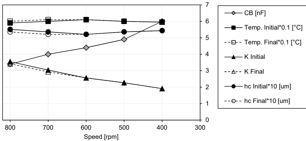
Figure 54. Change in evaluated parameters plotted as a function of decreasing rotational speed from 800 to 400 rpm. Parameters are shown after multiplying with a scalar factor to accommodate all information in the same figure.
