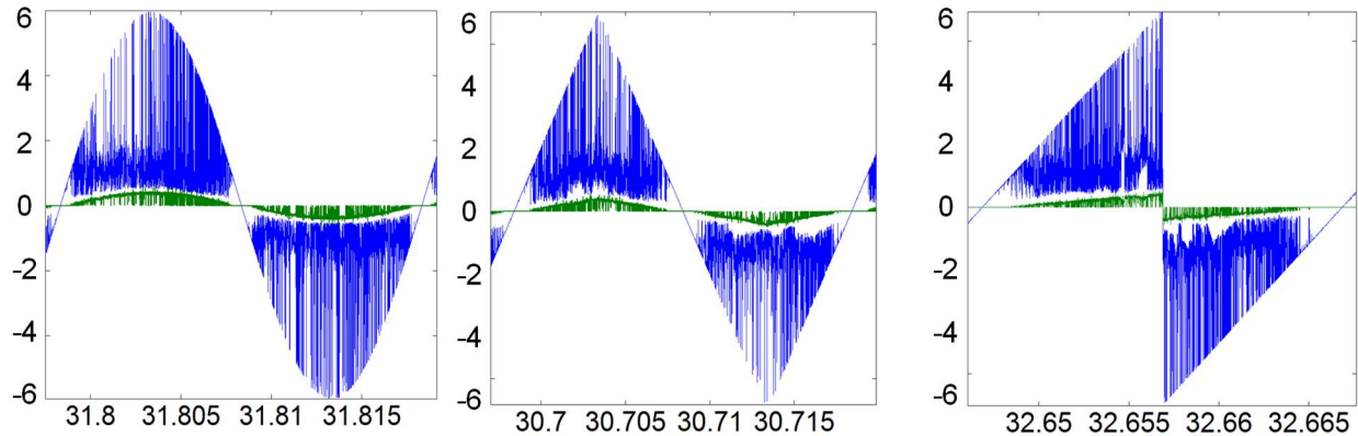
Figure 83. Bearing current activity (green) in lubricating film at V_{\text{peak}} of 6 V and frequency of 50 Hz at different voltage shapes (blue). It can be observed that the discharge bearing currents do not occur near the zero crossing of the alternating voltages. X-axis shows time in seconds for different measurements.
