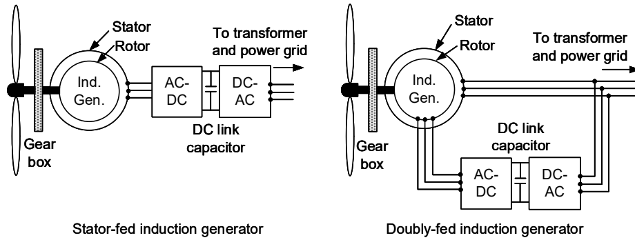
Figure 10. Simplified schematics of wind turbines in SFIG (left) and DFIG (right) arrangements. The converter is attached to stator-side for stator-fed arrangement, while it is attached to the rotor-side for doubly-fed arrangement.
