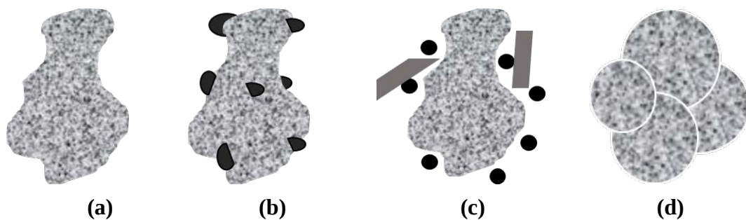
Figure 7: Schematic illustration of differently alloyed powder (a) pre-alloyed (b) diffusion bonded (c) admixed and (d) agglomerated powder.
