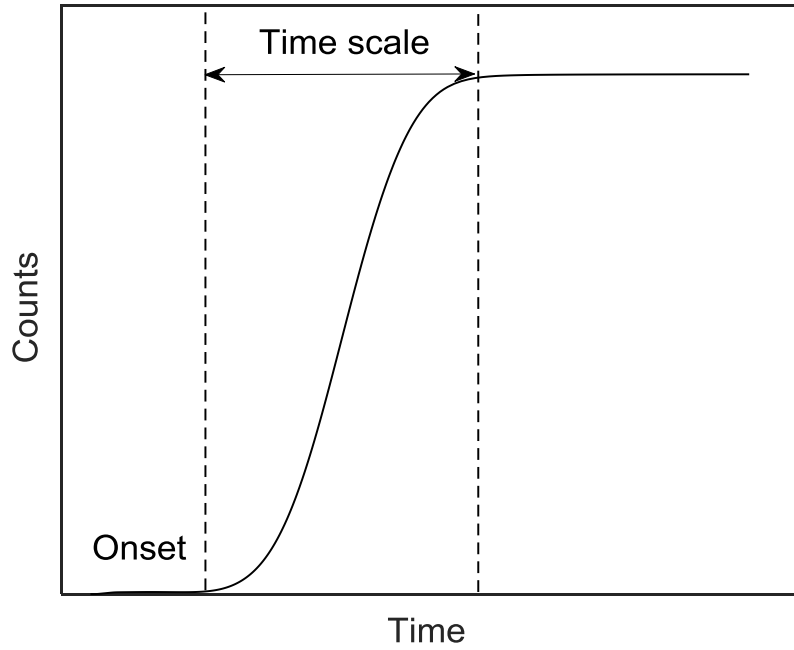
Figure 3-5. Schematic illustration of the onset of the formation of stable particles \geq 1 \mu\text{m} and the evolution of the following formation of particles on the micron scale, quantified as “counts” of the chords measured. The kinetics of the precipitation process levelled out, from which a time scale could be determined.
