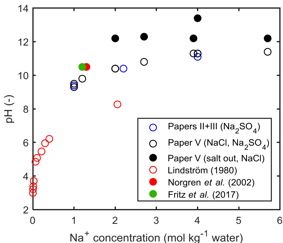
Figure 4-8. The pH value at the onset of the formation of particles \geq 1 \mu\text{m} or C.C.C. (literature sources) of \text{Na}^+ concentration.
