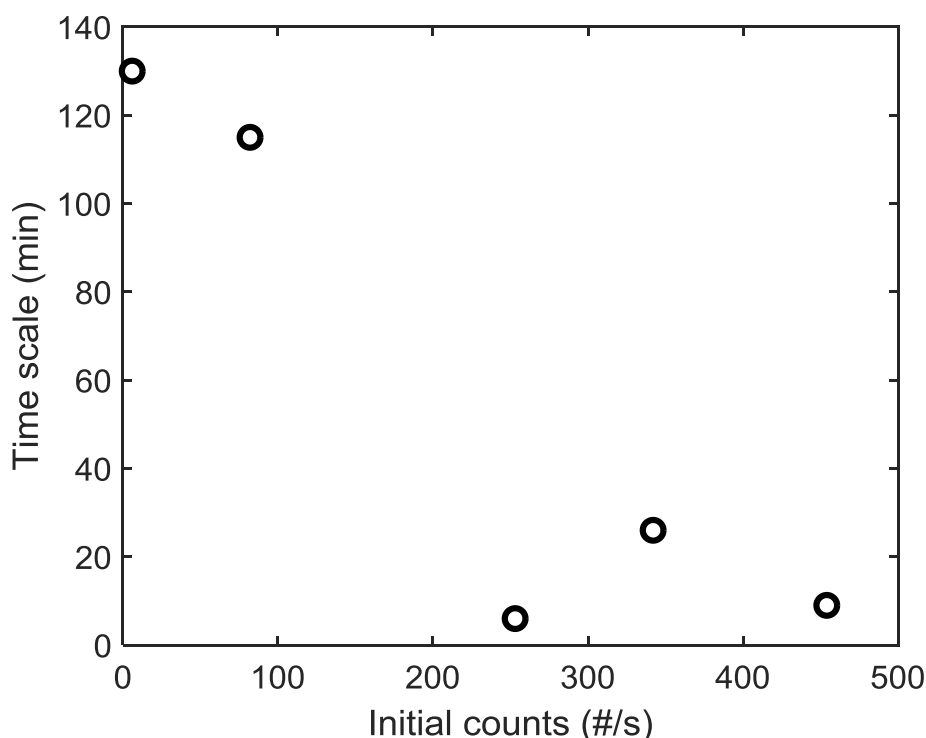
Figure 4-10. The time scale of precipitation vs. the initial counts of all particles \geq 1 \mu\text{m} prior to acidification. Salt added: \text{Na}_2\text{SO}_4 .
