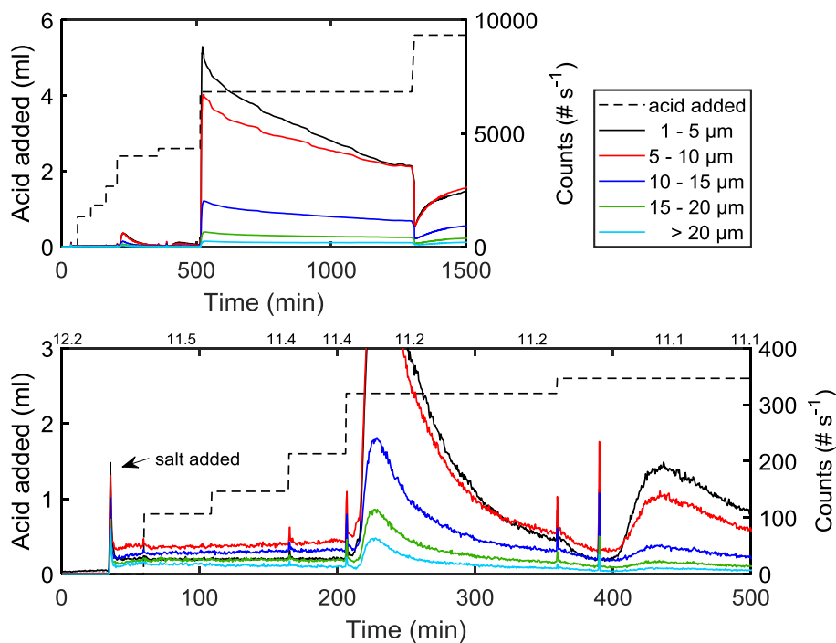
Figure 4-2. The course of precipitation. The line of numbers above the lower image are the pH values measured at 25 °C at various times throughout the experiment. Precipitation conditions: 65 °C, 3.9 mol Na + kg -1 water and Cl - as the anion.
