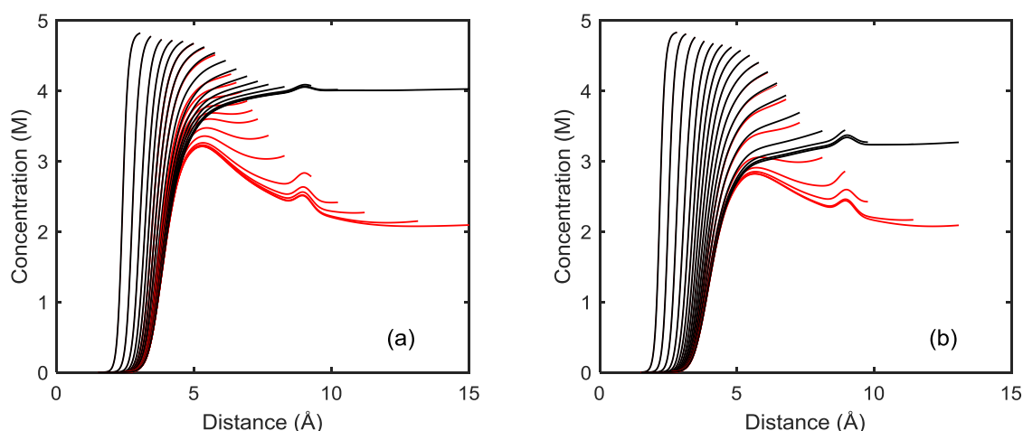
Figure 4-25. Concentration of ion vs. distance from the surface at various half-separation distances, D/2 (the end-points on right-hand side of each curve). Black curves: total ion concentration profiles. Red curves: \text{Na}^+ contribution made. Concentration of \text{Na}^+ in the bulk: 2.0 M. pOH: 2.0. (a) NaCl case. (b) \text{Na}_2\text{SO}_4 case.
