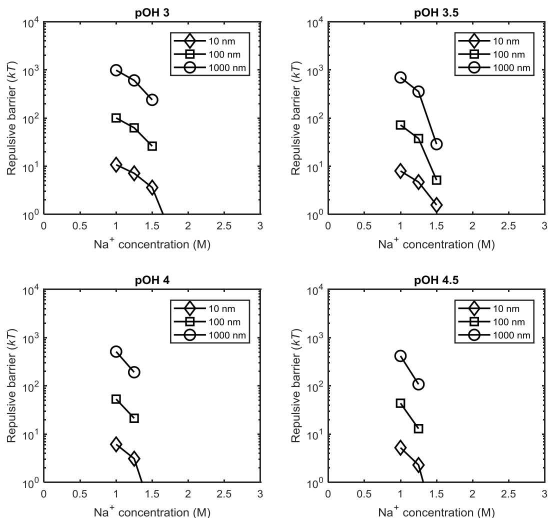
Figure 4-20. Pair interaction potentials between kraft lignin particles of radii 10, 100, and 1000 nm at various levels of salt concentration ( \text{Na}^+ ) with \text{Cl}^- as the anion in the added salt. The pOH is in the range 3-4.5 and the temperature is 65 °C. The content of phenolic and carboxylic groups ( \text{mol kg}^{-1} lignin) are 4.27 and 0.45, respectively.
