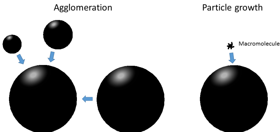
Figure 2-1. Schematic illustration of agglomeration (left) and particle growth (right).
