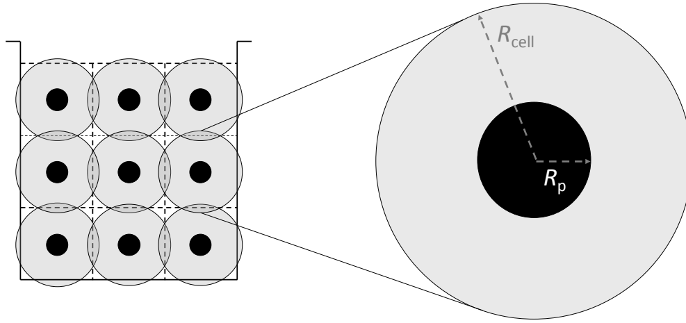
Figure 2-2. Schematic illustration of dispersed particles immersed in an electrolyte. The system is divided into equal spherical cells containing a concentric spherical particle. Each cell represent a Poisson-Boltzmann cell. R_{\text{cell}} and R_p are the radii of the PB cell and the particle, respectively.
