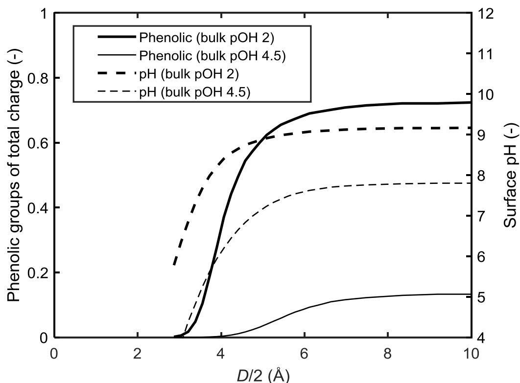
Figure 4-24. Fractions of charges from phenolic groups of total charge density (left y-axis) and surface pH (right y-axis) at various half separation-distances between two interacting kraft lignin particles/ macromolecules. Bulk conditions: pOH 2 and 4.5. Temperature: 65 °C.
