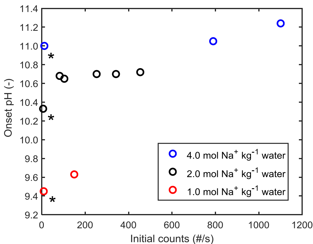
Figure 4-9. The onset pH of the formation of particles \geq 1 \mu\text{m} due to acidification at various concentrations of salt and amounts (initial counts) of pre-existing particles ( \geq 1 \mu\text{m} ) prior to acidification. Precipitation temperature: 45^\circ\text{C} . pH value at 25^\circ\text{C} . * The lignin solution was prefiltered prior to acidification. Salt added: \text{Na}_2\text{SO}_4 .
