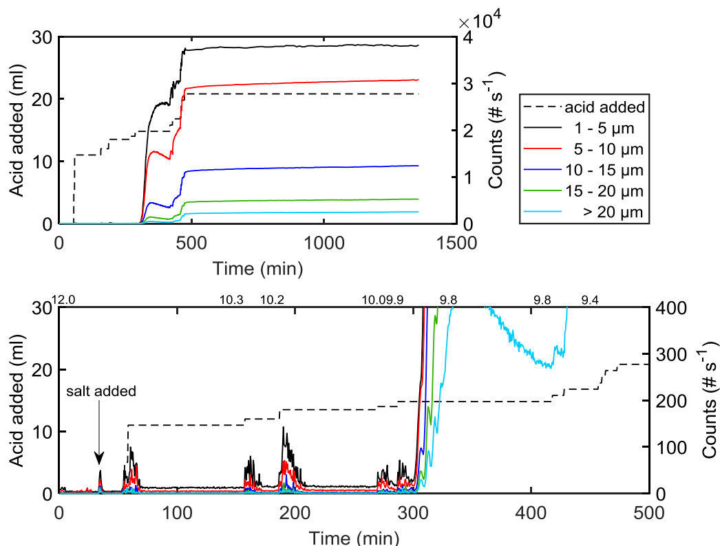
Figure 4-1. The course of precipitation. The line of numbers above the lower image are the pH values measured at 25^\circ\text{C} at various times throughout the experiment. Precipitation conditions: 65^\circ\text{C} , 1.2 \text{ mol Na}^+ \text{ kg}^{-1} water and \text{Cl}^- as the anion.
