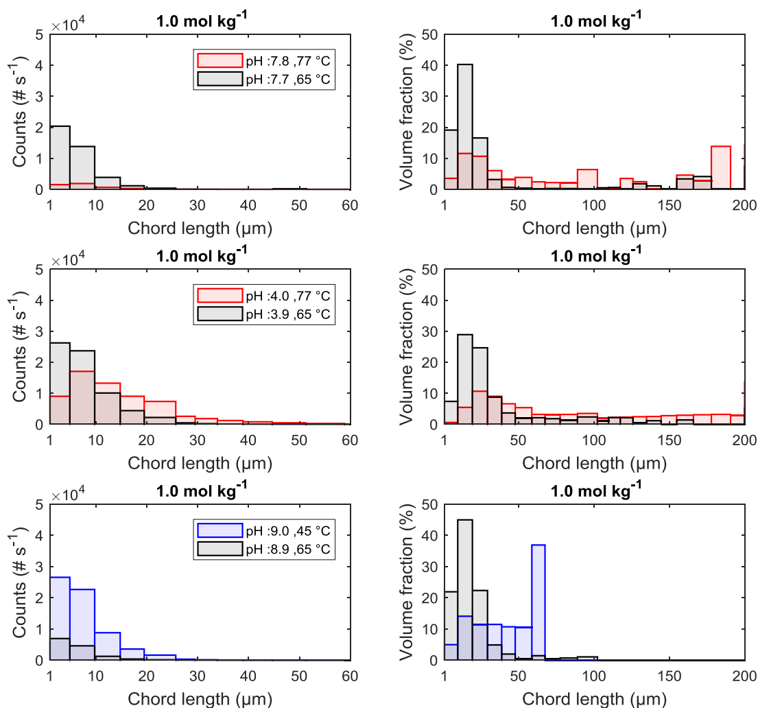
Figure 4-12. Number (counts) and volume-based chord length distributions at 45°C, 65 °C and 77 °C and at various pH levels. The \text{Na}^+ concentration was 1.0 \text{ mol kg}^{-1} water.
