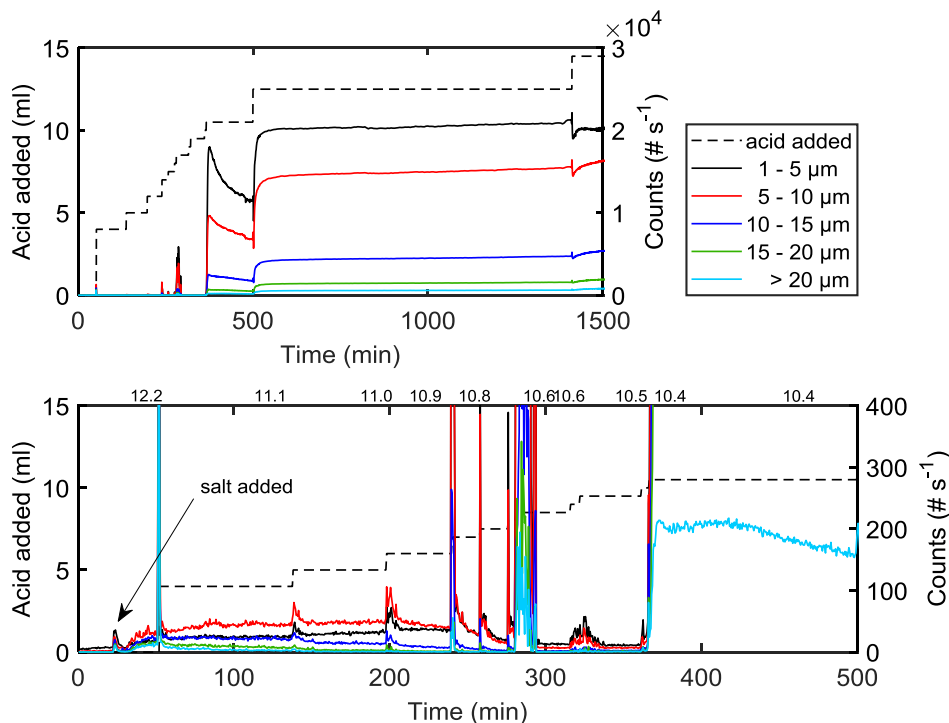
Figure 4-3. The course of precipitation. The line of numbers above the lower image are the pH values measured at 25 °C at various times throughout the experiment. Precipitation conditions: 65 °C, 2.0 mol Na + kg -1 water and Cl - as the anion.
