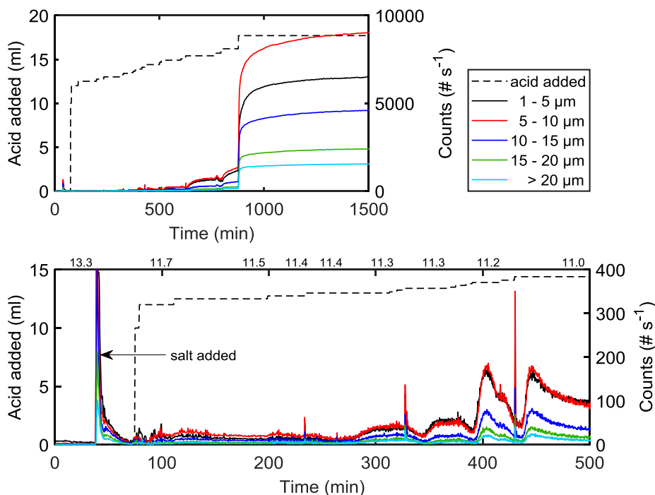
Figure 4-7. The course of precipitation. The line of numbers above the lower image are the pH values measured at 25 °C at various times throughout the experiment. Precipitation conditions: 45 °C, 4.0 mol Na + kg -1 water and SO 4 2- as the anion.
