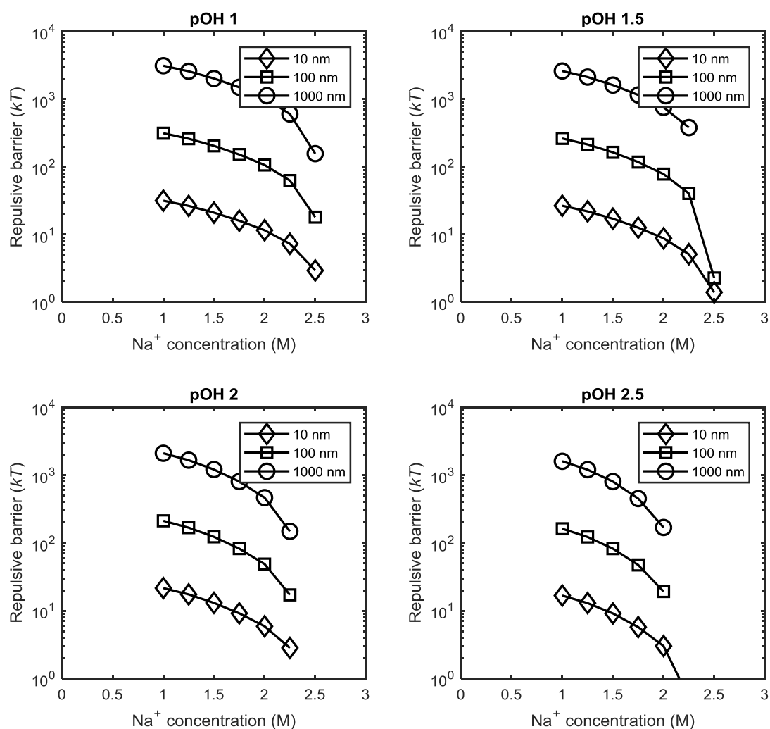
Figure 4-21. Pair interaction potentials between kraft lignin particles of radii 10, 100, and 1000 nm at various levels of salt concentration ( \text{Na}^+ ) with \text{SO}_4^{2-} as the anion in the added salt. The pOH is in the range 1-2.5 and the temperature is 65 °C. The contents of phenolic and carboxylic groups ( \text{mol kg}^{-1} lignin) are 4.27 and 0.45, respectively.
