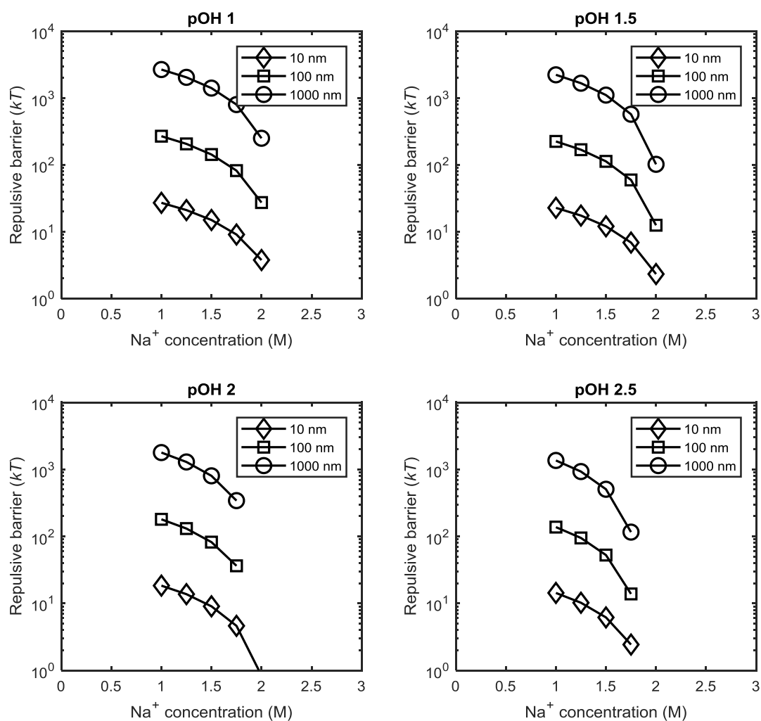
Figure 4-19. Pair interaction potentials between kraft lignin particles of radii 10, 100, and 1000 nm at various levels of salt concentration ( \text{Na}^+ ) with \text{Cl}^- as the anion in the added salt. The pOH is in the range 1-2.5 and the temperature is 65 °C. The contents of phenolic and carboxylic groups ( \text{mol kg}^{-1} lignin) are 4.27 and 0.45, respectively.
