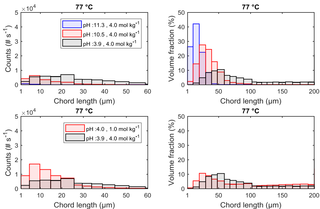
Figure 4-11. Number (counts) and volume-based chord length distributions at 77 °C. Upper panel: the influence of pH at 4 mol \text{Na}^+ \text{kg}^{-1} water. Lower panel: the influence of \text{Na}^+ concentration at about pH 4.
