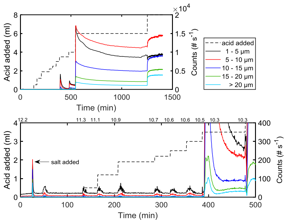
Figure 4-5. The course of precipitation. The line of numbers above the lower image are the pH values measured at 25 °C at various times throughout the experiment. Precipitation conditions: 65 °C, 2.0 mol Na + kg -1 water and SO 4 2- as the anion.
