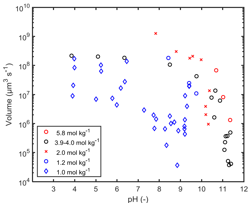
Figure 4-14. The total volume of particles ( \geq 1 \mu\text{m} ) measured per second with the FBRM vs. the pH level (measured at 25^\circ\text{C} ). The volume-estimates were based on the chord length distributions (see 3.4 Analysis of chord length counts).
