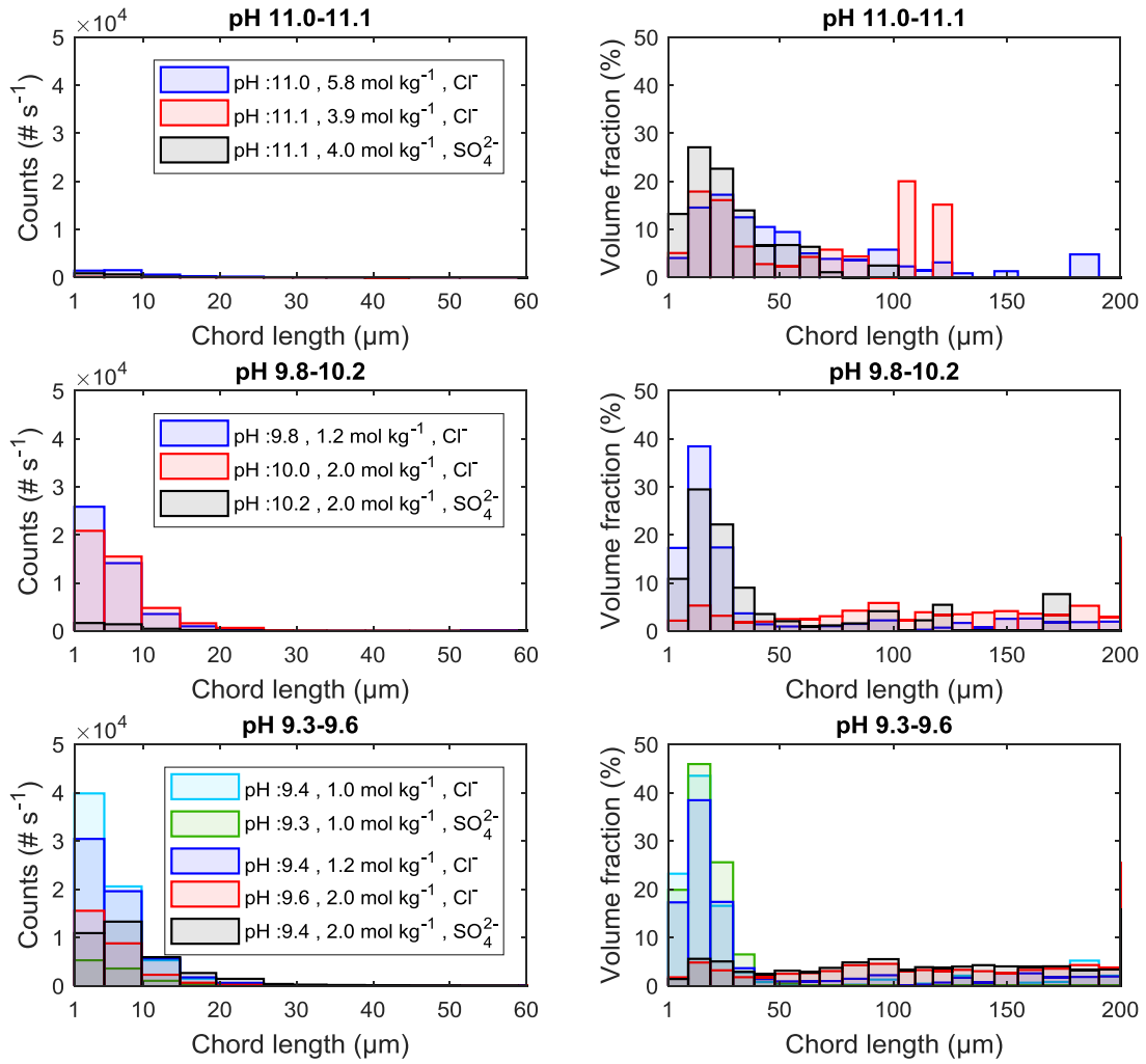
Figure 4-13. Number (counts) and volume-based chord length distributions at 65 °C. The influence of \text{Na}^+ concentration and anionic type ( \text{SO}_4^{2-} and \text{Cl}^- ) is shown at three pH levels ( \sim 11 , \sim 10 , and \sim 9.4 ).
