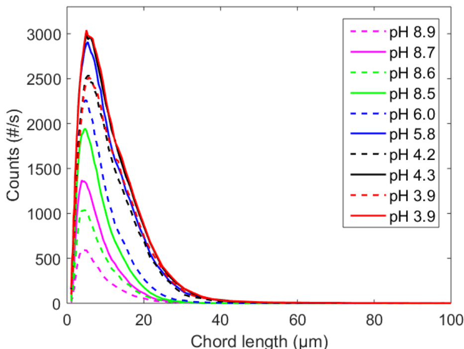
Figure 4-18. Comparison of chord length distributions with (dashed line ---) and without (full line —) xylan added. \text{Na}^+ concentration: 1.0 \text{ mol kg}^{-1} water. Precipitation temperature: 65^\circ\text{C} .
