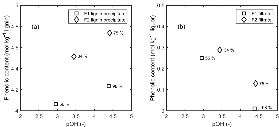
Figure 4-26. Contents of phenolic groups (a) in the precipitated kraft lignin from black liquor factions (30 wt% dry content) and (b) in the remaining liquor, vs. the pOH (from Paper IV). The gravimetric yields at the corresponding conditions are given in percentage. F1 and F2 are a high and medium molecular weight fraction, respectively, with respect to the original unfractionated softwood black liquor.
