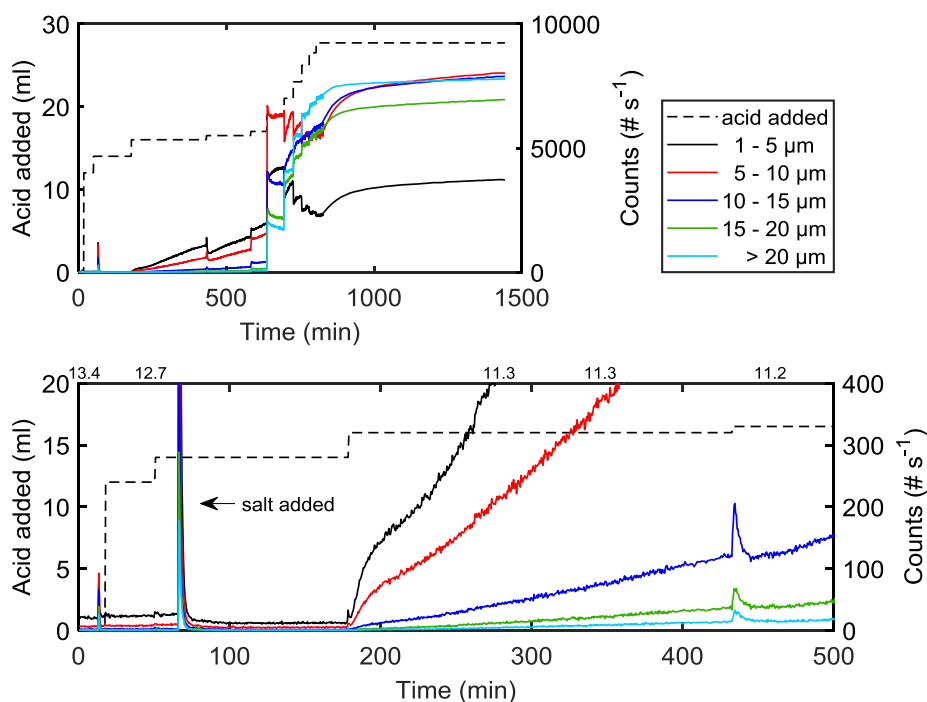
Figure 4-6. The course of precipitation. The line of numbers above the lower image are the pH values measured at 25 °C at various times throughout the experiment. Precipitation conditions: 77 °C, 4.0 mol Na + kg -1 water and SO 4 2- as the anion.
