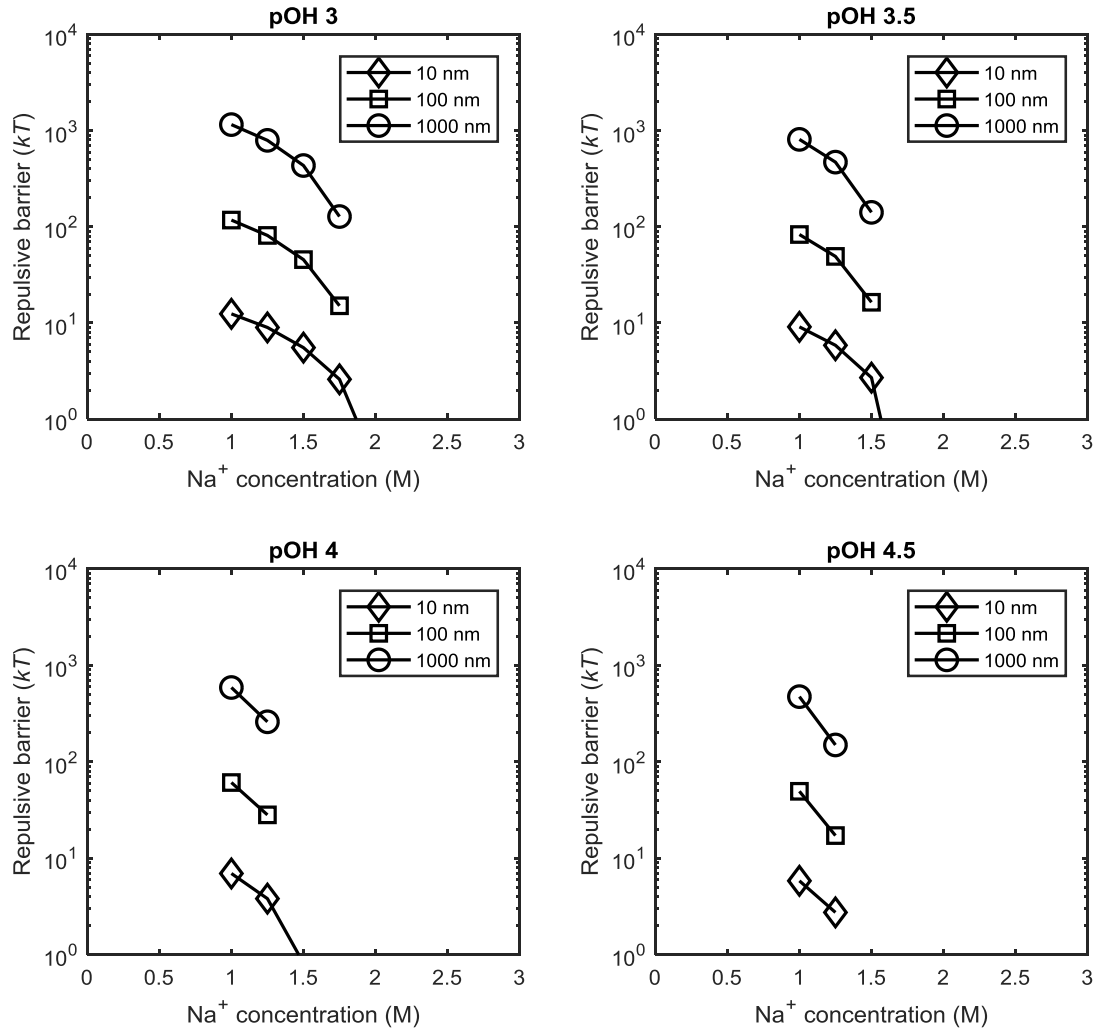
Figure 4-22. Pair interaction potentials between kraft lignin particles of radii 10, 100, and 1000 nm at various levels of salt concentration ( \text{Na}^+ ) with \text{SO}_4^{2-} as the anion in the added salt. The pOH is in the range 3-4.5 and the temperature is 65 °C. The contents of phenolic and carboxylic groups ( \text{mol kg}^{-1} lignin) are 4.27 and 0.45, respectively.
