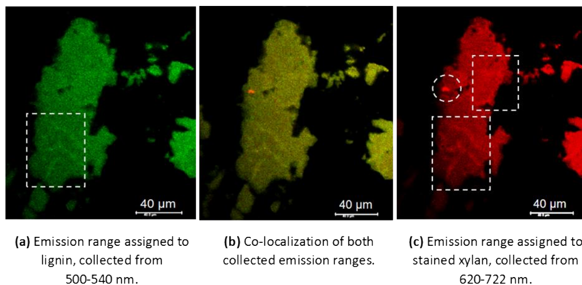
Figure 4-15. Images of the intensity landscape of emitted light collected in different wavelength intervals: (a) light emission range collected predominantly from auto-fluorescent lignin; (b) superimposed images of collection ranges assigned to lignin and dyed/stained xylan and (c) wavelength span corresponding to the strongest emittance from dyed xylan.
