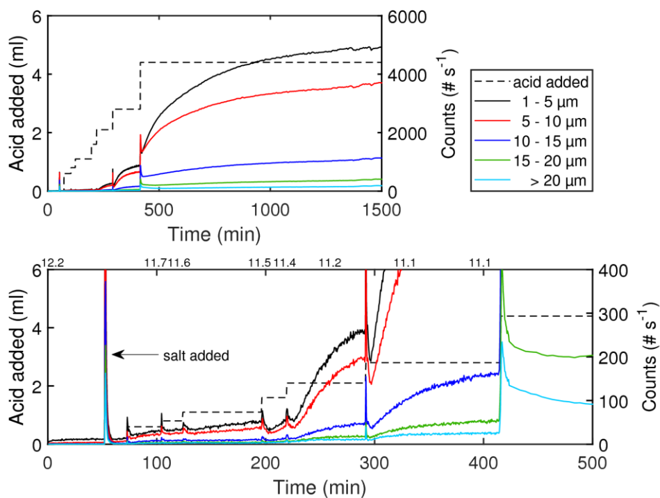
Figure 4-4. The course of precipitation. The line of numbers above the lower image are the pH values measured at 25 °C at various times throughout the experiment. Precipitation conditions: 65 °C, 4.0 mol Na + kg -1 water and SO 4 2- as the anion.
