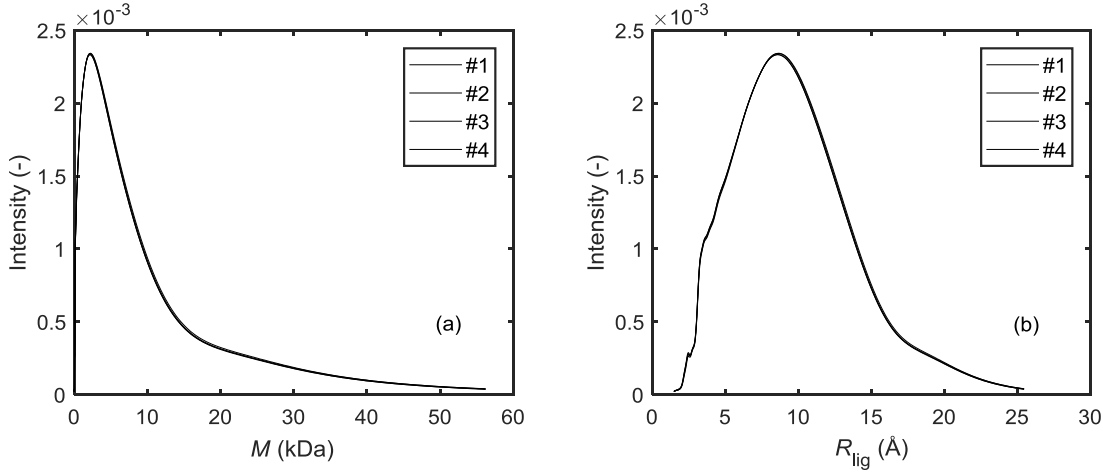
Figure 3-1. (a) Molecular weight and (b) estimated macromolecular size distributions of the initial kraft lignin powder sampled four times (#1-4). The average M_n and M_w are 3.1 and 11.3 kDa, respectively.
