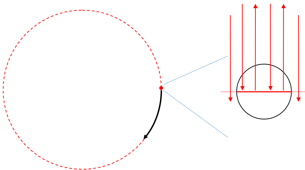
Figure 3-4. Schematic diagram of the Focused Beam Reflectance Measurement (FBRM) technique. The laser beam is focused on a point located just outside the probe window in the fluid being analysed. The focal point moves along a circular path at a fixed speed and, as a particle passes it, back-scattering of light occurs. This is returned to the probe and measured by the equipment.
