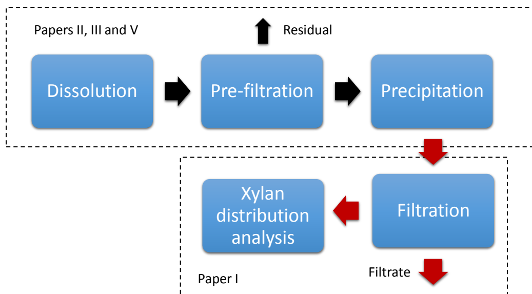
Figure 3-2. Overview of steps in the experimental procedure.
