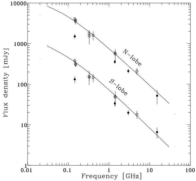
Fig. 5. DYNAGE fits (solid lines) to the total intensity spectra of the north-west and south-east lobes (open circles), and the spectral points of the hotspot regions (filled dots; not used in the fits). Note that the north-west lobe flux density scale is shifted one decade up in relation to the given ordinate scale.
