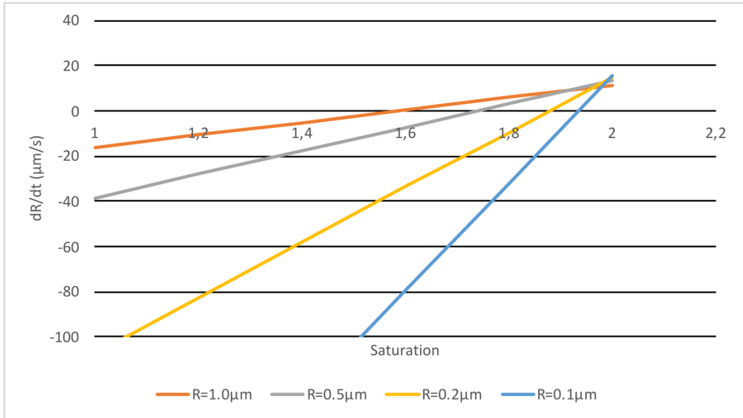
Fig 1. Rate of change in radius ( R ) due to diffusion for a clean air bubble in water, with a surface tension of 72\text{N/cm} and at 293\text{K} . Calculated from eq (15) in (58) . A negative value means a shrinking bubble, a positive value means a growing bubble.
