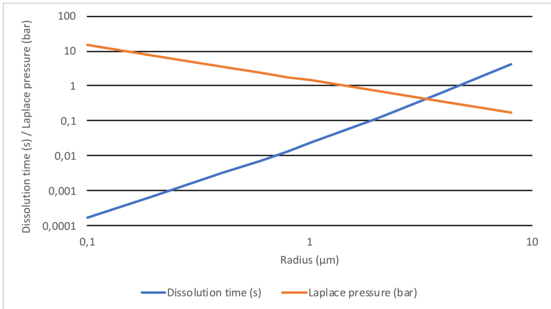
Fig 2. Blue line: Time for complete dissolution of an air bubble in water with 100% air saturation, a surface tension of 72\text{N/cm} and at 293\text{K} . Calculated from eq (17) in (58) . Orange line: Laplace pressure under the same conditions. Both axes are logarithmic.
