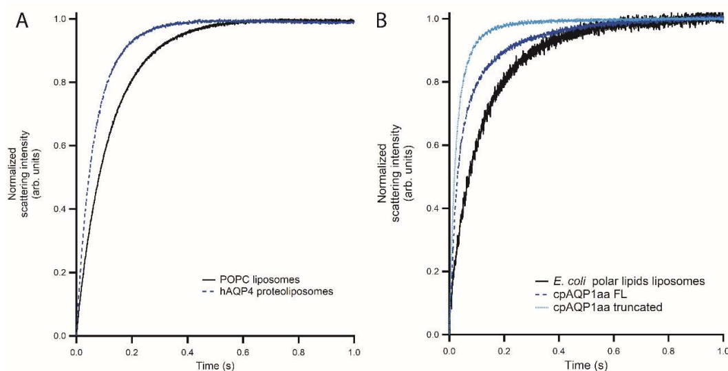
Figure 6: Aquaporin functionality assessments using stopped-flow light scattering. (A) hAQP4-containing POPC proteoliposomes (dashed, blue) compared to POPC liposomes (solid, black). (B) Full-length cpAQP1-containing E. coli polar lipid proteoliposomes (dashed, blue) compared to truncated cpAQP1-containing E. coli polar lipid proteoliposomes (dotted, light blue) and E. coli polar lipid liposomes (solid, black).
