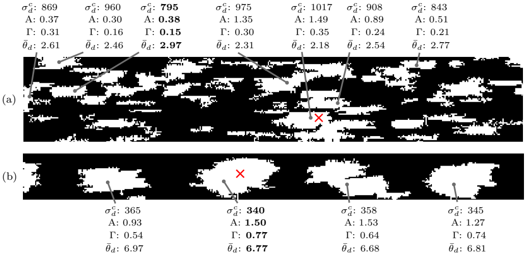
Figure 4.5: Figure from Paper E. Examples of defects assessed with the defect severity model for (a) a sample with random fibre waviness and (b) a sample with periodic fibre waviness. The bold face values represent the critical values with lowest strength ( \sigma_d^c = \sigma_{cr}^c ). Strength values \sigma_d^c are reported in MPa and misalignment angles \theta_d in degrees. The cross indicates failure initiation region based on the FE model. Strength values that are not shown are higher than the presented ones.
