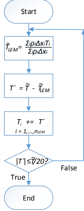
Figure 1.9: Steps of correcting the temperature in a LEM domain. Here T_i is the temperature of LEM cell i and n_{LEM} is the total number of LEM cells. The temperature difference T' is a difference between the LES temperature \tilde{T} and the Favre-averaged LEM temperature \tilde{T}_{LEM} .
