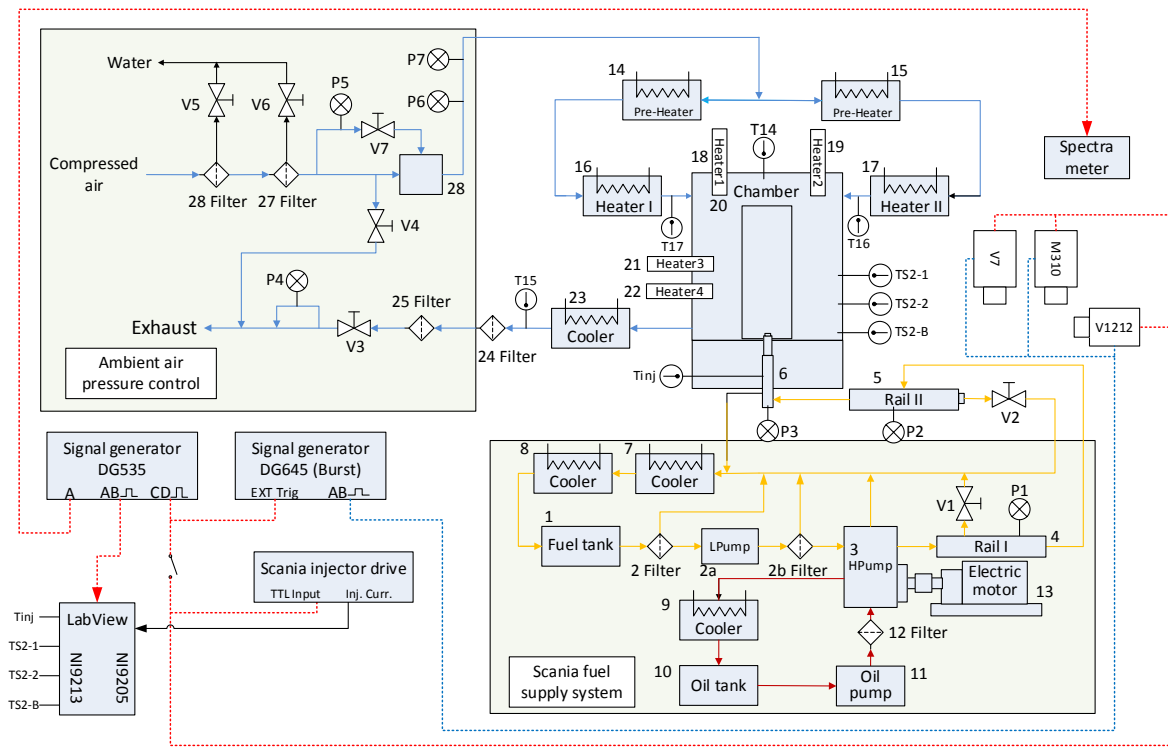
Figure 3-6 Schematic of the high pressure high temperature constant volume combustion chamber experimental setup
