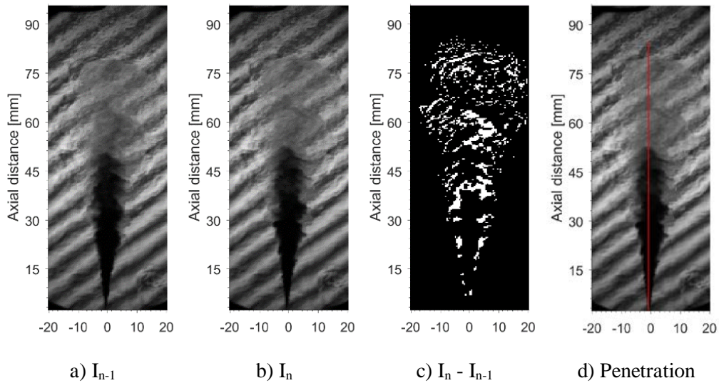
Figure 3-10 Vapour phase spray penetration processing procedure. Diesel fuel injection at injection pressure of 120 MPa, ambient temperature of 623 K, gas density of 26 kg/m 3 and 2 ms after the electronic start of injection. Red line is vapour phase penetration
