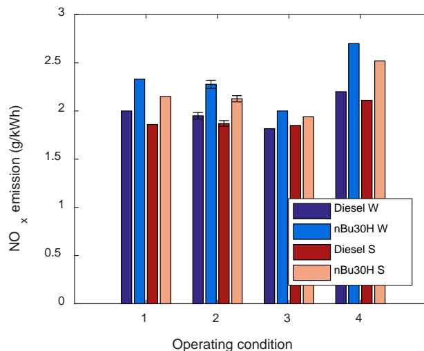
Figure 4-17 Conventional CI combustion NO x emissions generated using the wave and standard pistons at various operating points in the HD engine.
