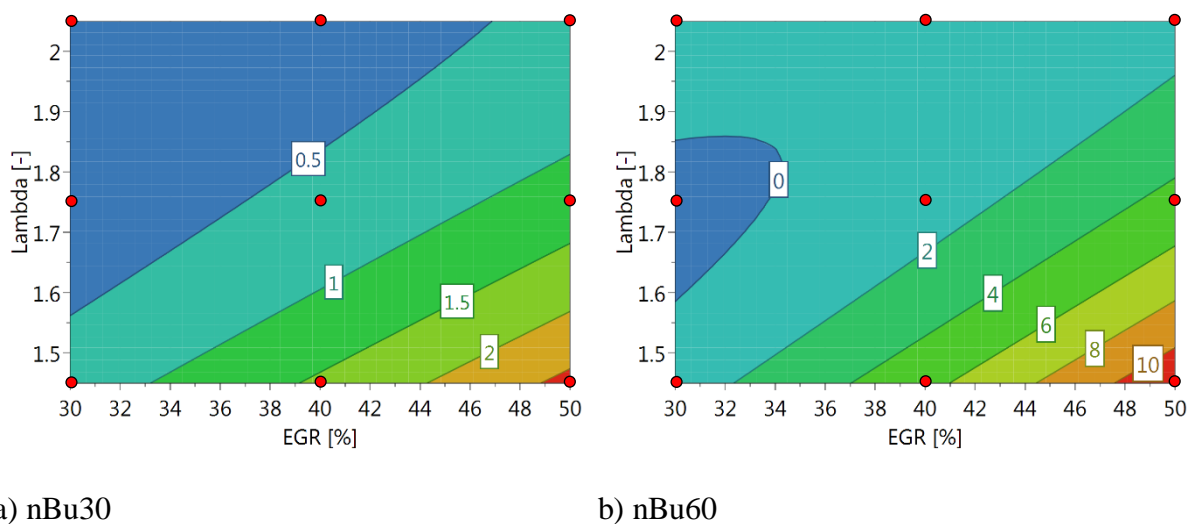
Figure 4-22 Partially premixed combustion indicated CO emissions of a) nBu30 and b) nBu60 at the engine speed of 1280 rpm and IMEP of 0.96 MPa in the LD engine.
