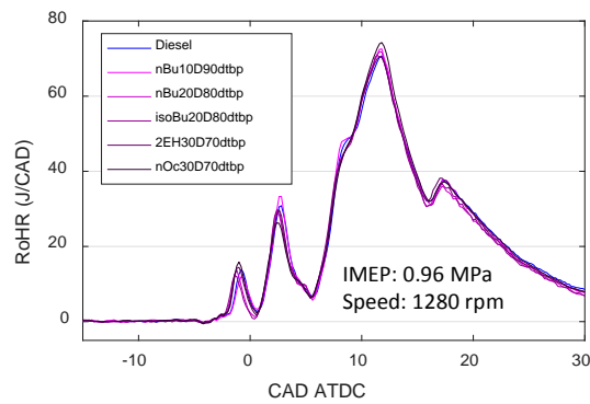
c) Alcohol and Diesel blends with DTBP in the LD engine
