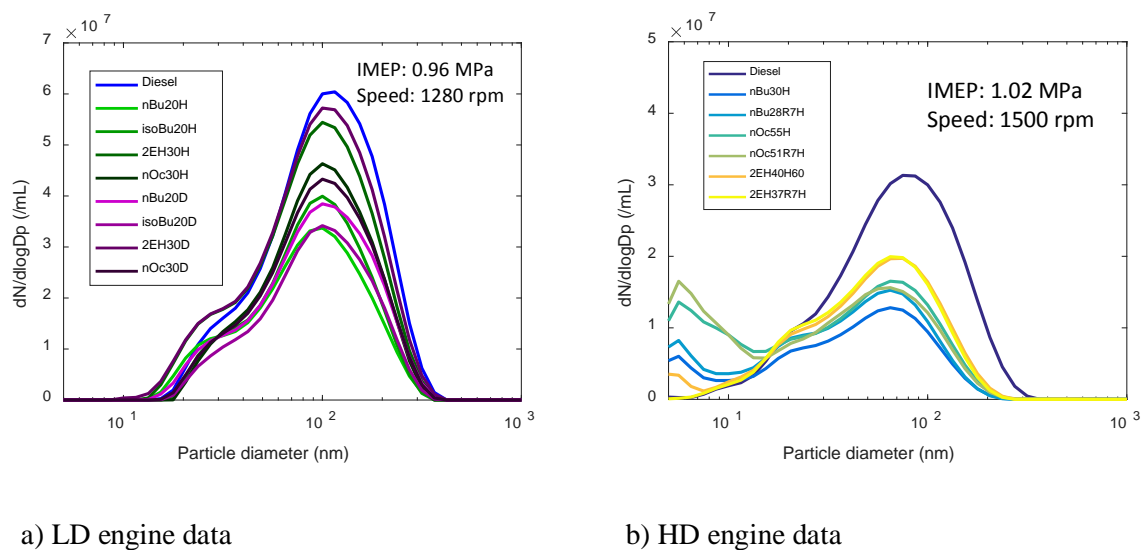
Figure 4-14 Particulate matter size distributions in the (a) LD and (b) HD engines. (Paper II)
