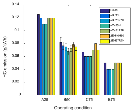
Figure 4-24 HC emissions of fossil-free fuels at various operating conditions in the HD engine.
