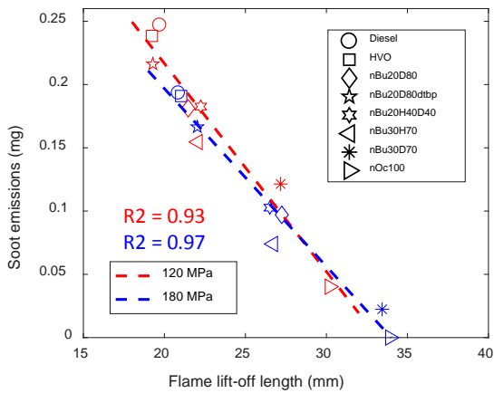
a) Soot emissions versus flame lift-off length
