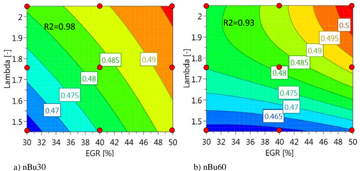
Figure 4-8 Indicated thermal efficiency of partially premixed combustion with a) nBu30 and b) nBu60 at an engine speed of 1280 rpm and an IMEP of 0.96 MPa in the LD engine. (Paper III)
