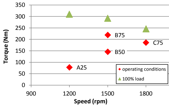
Figure 3-4 Operating conditions of the HD engine
