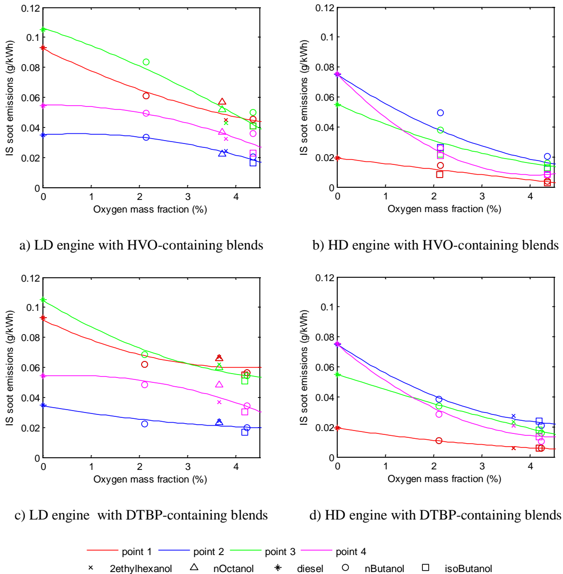
Figure 4-9 Conventional CI combustion indicated soot emissions plotted against the fuel’s oxygen mass fraction at four operating points for (a) LD and (b) HD engines with HVO-containing blends, and (c) LD and (d) HD engines with DTBP-containing blends. (Paper I and II)
