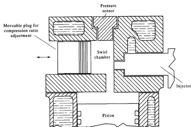
Figure 2-4 Combustion chamber of a CFR engine [60]
