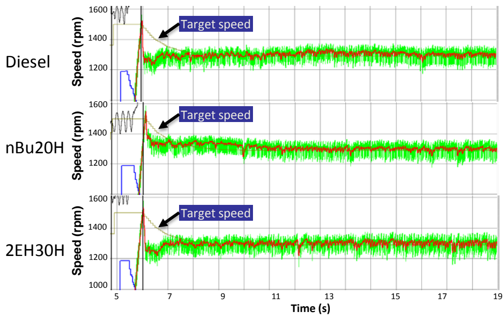
Figure 4-27 Engine speed during cold start experiments. Taken from Volvo Cars' report.
