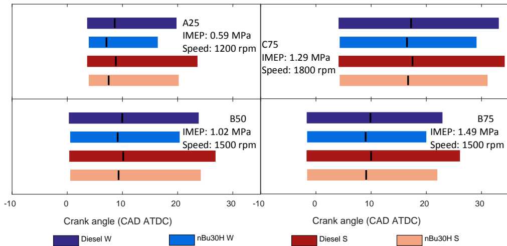
Figure 4-3 Conventional CI combustion durations (defined as the period between SOC and CA90) achieved using standard and wave piston designs for Diesel and nBu30H at the A25, B50, C75, and B75 operating points.
