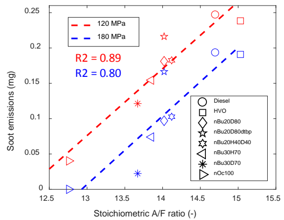
d) Soot emissions versus stoichiometric A/F ratio
