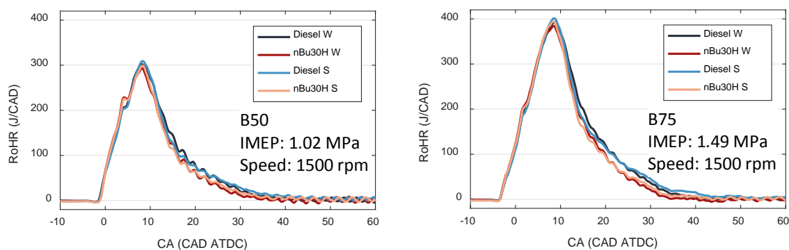
Figure 4-2 Conventional CI combustion rate of heat release curves of Diesel and nBu30H using wave piston and standard omega piston in the HD engine at the B50 and B75.
