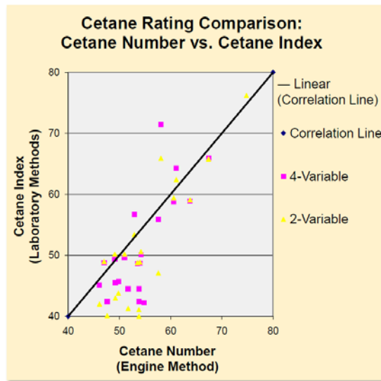
Figure 2-7 Comparison of cetane index and cetane number (CFR) [74]
