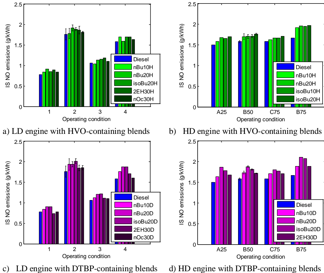
Figure 4-16 Conventional CI combustion indicated specific NO emissions generated under various conditions with HVO-containing blends in the (a) LD and (b) HD engines, and with DTBP-containing blends in the (c) LD and (d) HD engines. (Paper II)
