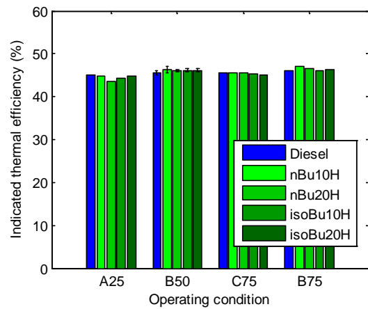
b) Alcohol, Diesel and HVO blends in the HD engine
