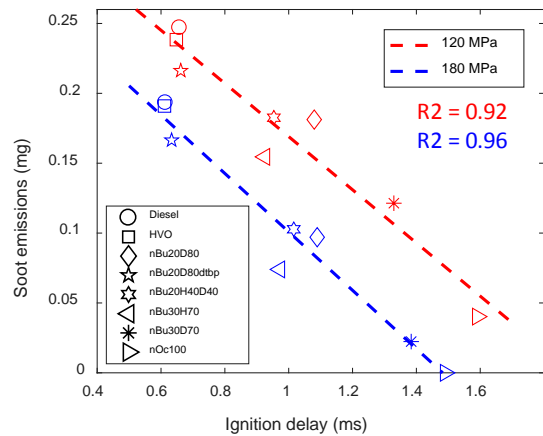
b) Soot emissions versus ignition delay
