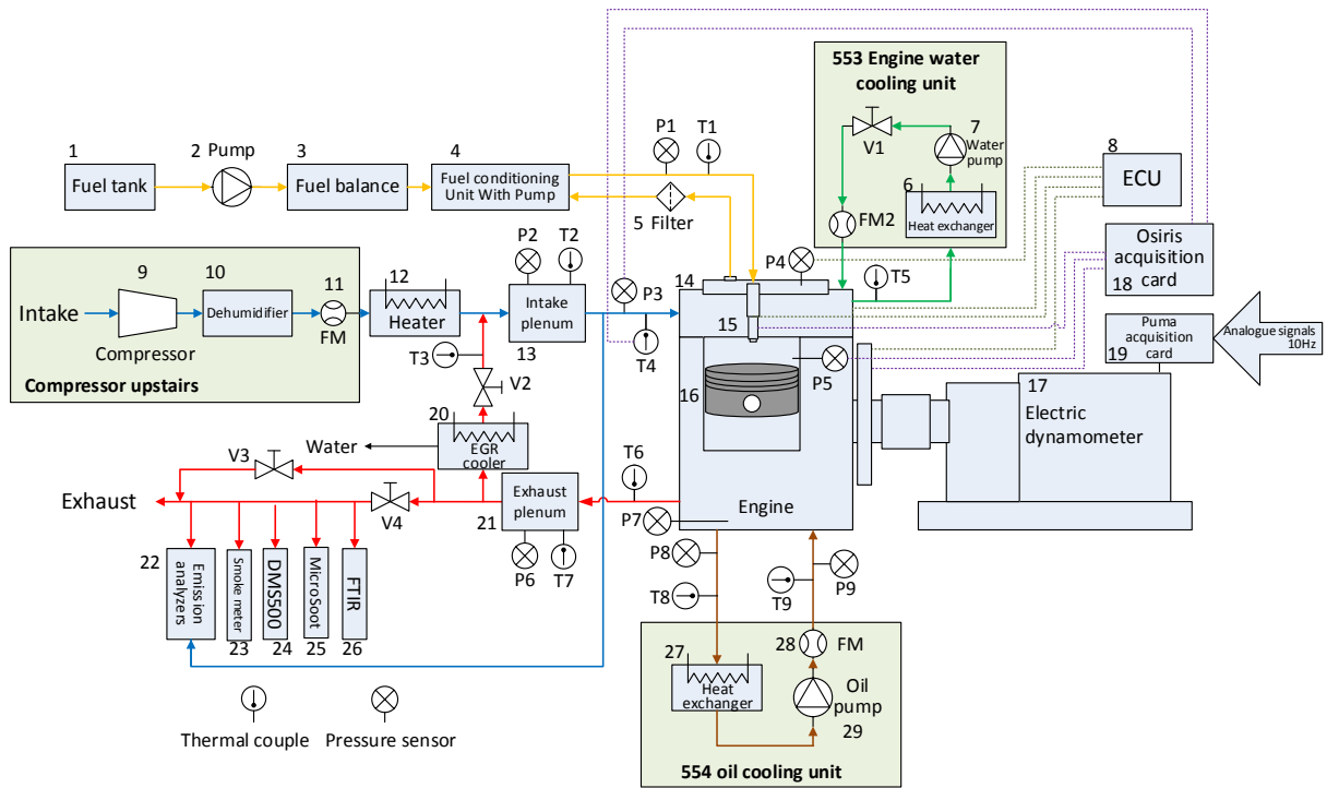
Figure 3-3 Schematic of the HD engine experimental setup
