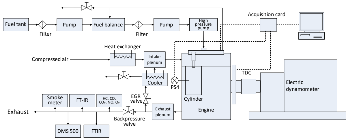
Figure 3-5 Schematic of the LD engine experimental setup
