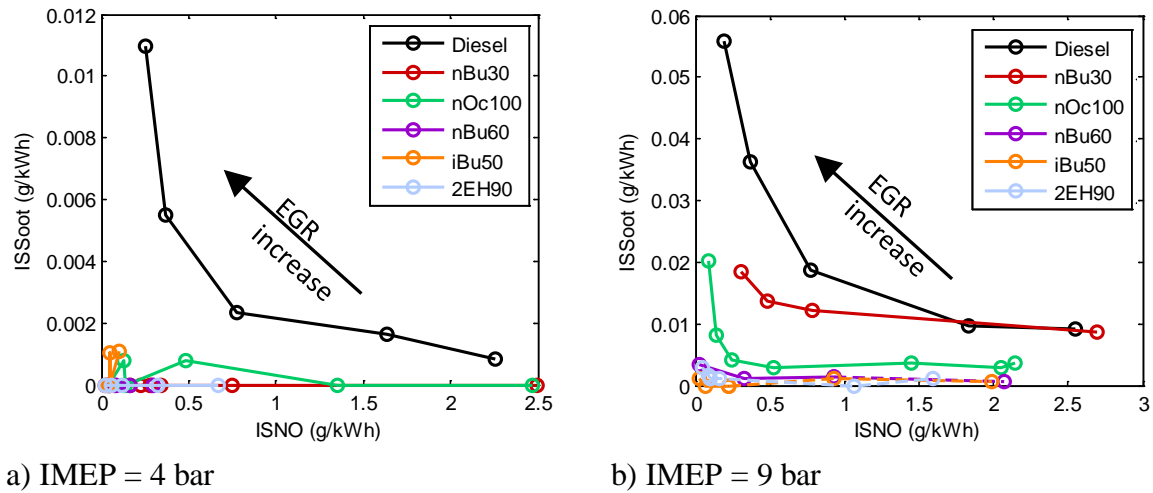
Figure 4-18 Partially premixed combustion soot-NO trade-off curves as functions of the EGR at a) 4 bar IMEP and b) 9 bar IMEP. In all cases, CA50 = 8 CAD ATDC or the earliest possible value, and lambda = 2.0. (Paper III)
