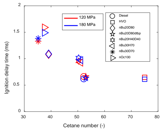
Figure 4-13 Ignition delay as a function of CN in the constant volume chamber
