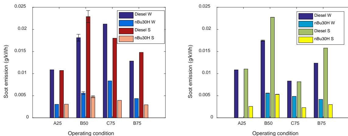
b) Production engine settings but fixed CA50 = 8 CAD ATDC
