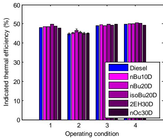
c) Alcohol and Diesel blends with DTBP in the LD engine
