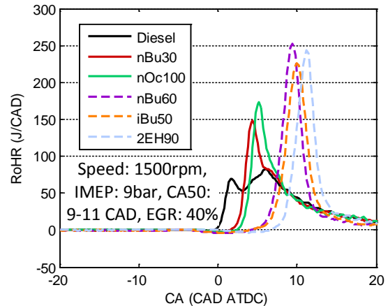
Figure 4-4 Rate of heat release curves for the tested low CN fuels at 4 bar IMEP (Paper III) Figure 4-5 Rate of heat release curves for the tested low CN fuels at 9 bar IMEP (Paper III)
