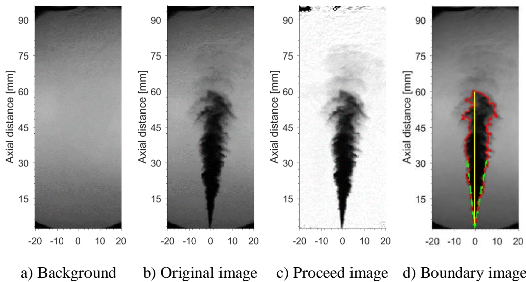
Figure 3-9 Liquid phase spray penetration and spray cone angle processing procedure. Diesel fuel injection at injection pressure of 120 MPa, ambient temperature of 623 K, gas density of 26 kg/m 3 and 2 ms after the electronic start of injection. Red line is liquid phase boundary, yellow line is penetration and green dash lines show the spray cone angle.
