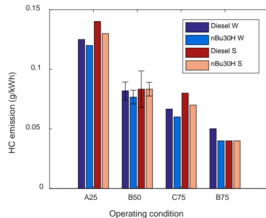
Figure 4-25 The wave and standard pistons' effects on HC emissions.
