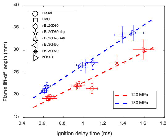
Figure 4-12 Flame lift-off length as a function of the ignition delay time (Paper IV)
