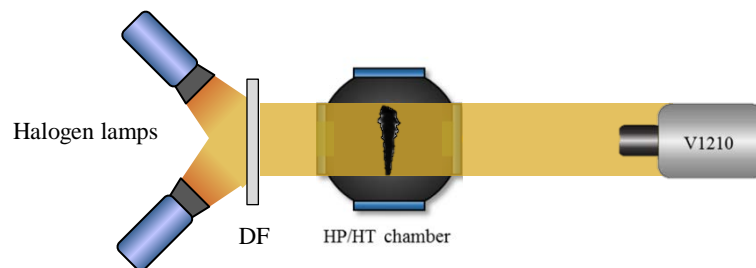
Figure 3-7 Optical set-up with the constant volume combustion chamber for non-combusting conditions
