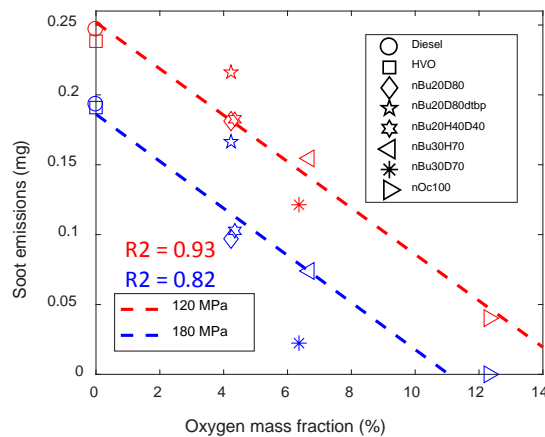
c) Soot emissions versus oxygen mass fraction in the fuels
