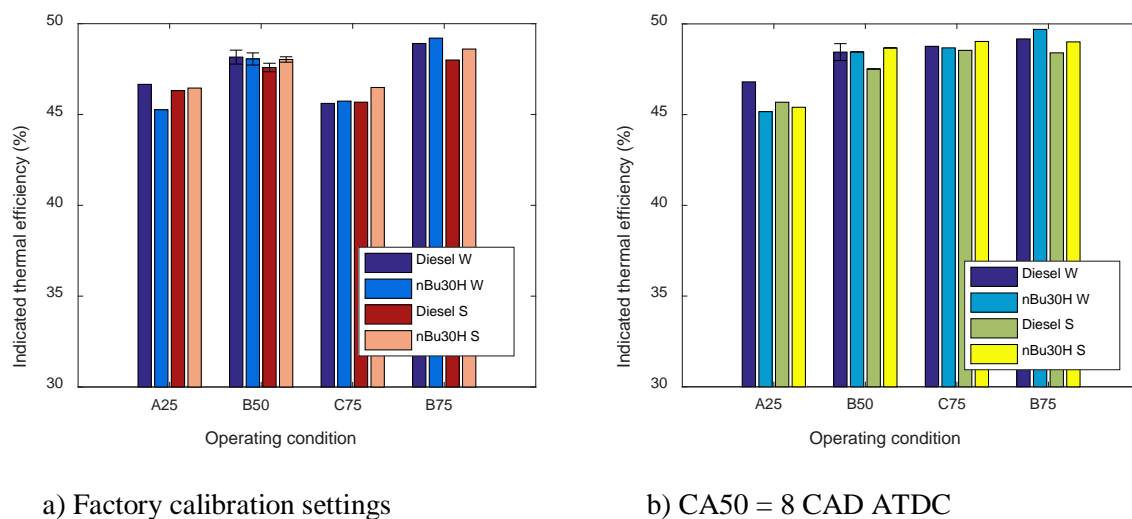
Figure 4-7 Conventional CI combustion indicated thermal efficiencies when using Diesel and nBu30H in the HD engine with the wave piston and the standard piston at a) factory calibration settings and b) with a fixed CA50 of 8 CAD ATDC.
