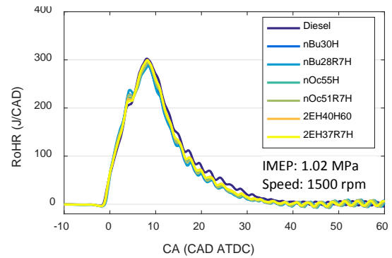
f) Fossil-free blends in the HD engine
