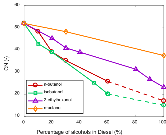
Figure 3-1 CN values for different alcohol/Diesel blends as functions of their alcohol content.
