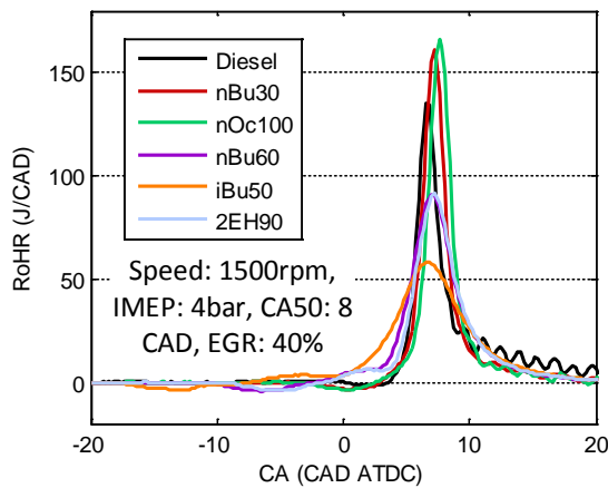
Figure 4-4 Rate of heat release curves for the tested low CN fuels at 4 bar IMEP (Paper III) Figure 4-5 Rate of heat release curves for the tested low CN fuels at 9 bar IMEP (Paper III)
