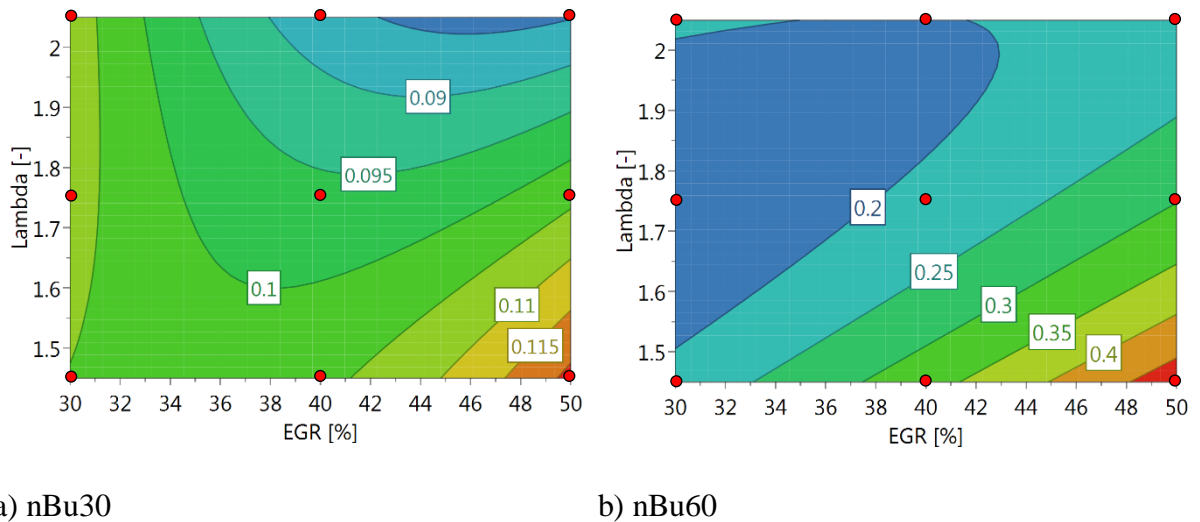
Figure 4-26 Partially premixed combustion indicated HC emissions of a) nBu30 and b) nBu60 at an engine speed of 1280 rpm and IMEP of 0.96 MPa in the LD engine.
