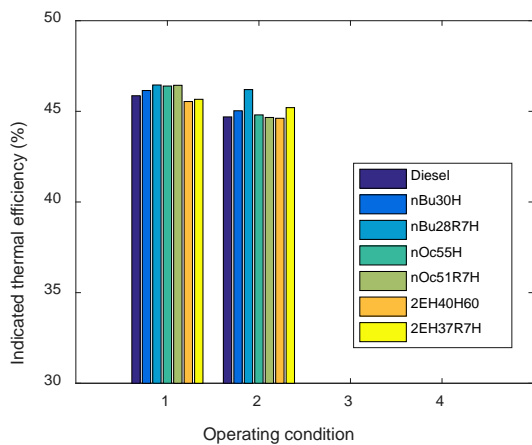
e) Fossil-free blends in the LD engine
