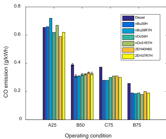
Figure 4-20 CO emissions of fossil-free fuels under various operating conditions.
