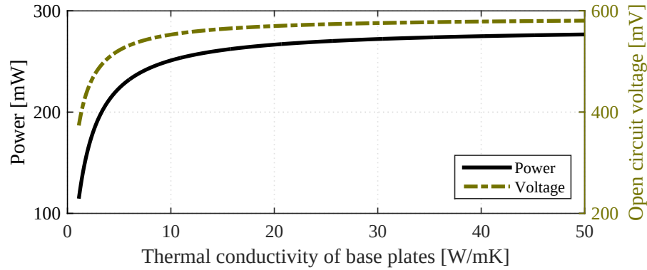
Figure 2.5: The power output and open circuit voltage of a 7-couple device with 1 mm thick base plates as a function of the thermal conductivity of the base plates. Alumina has a thermal conductivity of 7 W m -1 K -1 at 800°C compared to SiC with 48 W m -1 K -1 . The thermal gradient of the environment is 200°C.
