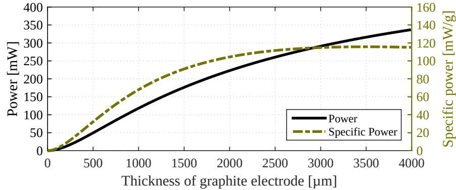
Figure 2.11: The power output and specific power of a 17-couple harvester as a function of the thickness of the graphite electrodes. Maximum specific power is achieved when the electrodes are approximately 3500 \mu\text{m} .
