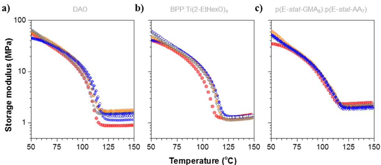
Figure 47: Storage modulus G' for p(\text{E-stat-GMA}_8) samples cured for 5 minutes at 200 °C with a) DAO b) BPP:Ti(2-EtHexO) 4 and c) p(\text{E-stat-AA}_7) and aged in air and room temperature for 1 (●), 90 (●), 180 (◇), 270 (◆), 360 (●), 450 (○) and 540 (◆) days.
