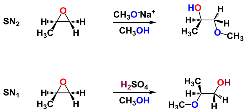
Figure 11: Epoxy ring opening reactions, \text{SN}_1 and \text{SN}_2 .
