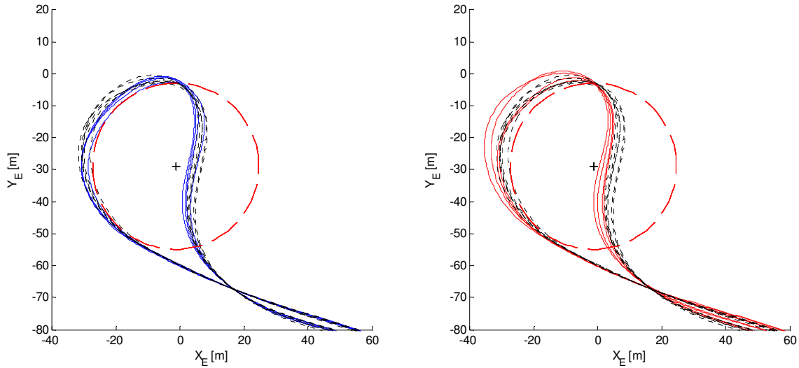
Figure 3: Vehicle trajectories in global ( X_E , Y_E ) coordinates showing off-tracking from the reference circle (dashed red lines) for PPR (left, solid lines) and DYC (right, solid lines) relative to the uncontrolled vehicle (dashed lines).
