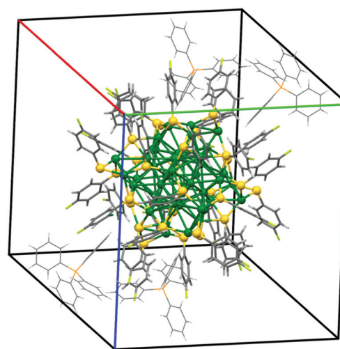
Fig. 4 C_1 unit cell reconstructed using XRD of single crystals at RT. Lattice parameters: (red line) a = 20.746(4) \text{ \AA} , (green line) b = 21.188(4) \text{ \AA} , (blue line) c = 22.462(4) \text{ \AA} , \alpha = 94.71(3)^\circ , \beta = 115.14(3)^\circ and \gamma = 117.54(3)^\circ (space group \bar{1} , volume 7433(4) \text{ \AA}^3 ). The total volume of solvent accessible voids amounts to 289 \text{ \AA}^3 .
