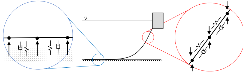
Fig. 2. Outline of the lumped-mass modelling approach.
