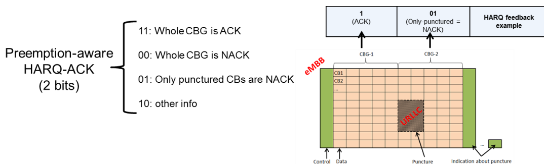
Figure B.3.3: Proposed PI-aware HARQ-ACK feedback. 2 feedback bits example.
