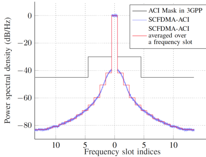
Figure B.10.1 Different ACI models.
