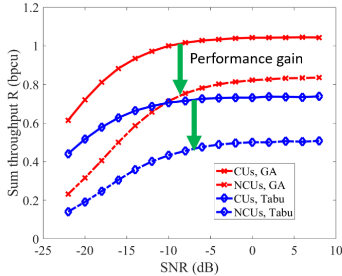
Figure B.2.2: The optimized end-to-end sum throughput of all users with cooperative and non-cooperative cases for the GA and Tabu method.
