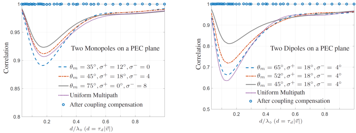
Figure B.1.1: Normalized temporal correlation vs. the element separation in double-exponential non-uniform multipath environments
