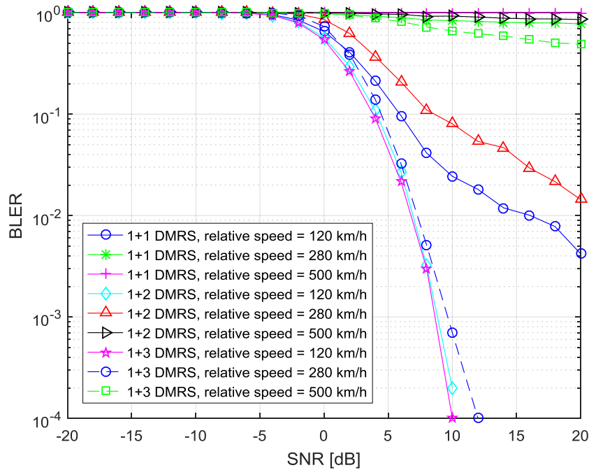
Figure B.12.1: BLER vs. SNR for single link V2V channel, QPSK modulation and code rate \frac{1}{2} , with different NR eMBB DMRS structures and different relative speeds between the transmitter and the receiver. ‘1+n DMRS’ denotes 1 front-loaded DMRS symbol and n additional DMRS symbols (n=1,2,3).
