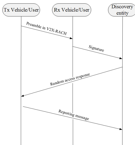
Figure 3.3-8 – Message exchange for the proposed V2X discovery scheme.
