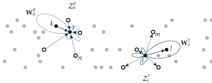
Figure 3.3-1: Illustration of transmit- and receive side nulling sets, here denoted by (Z_{ij}^T) and (Z_{lk}^R) .
