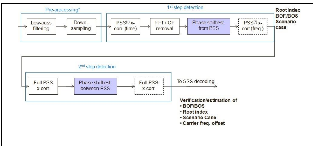
Figure 3.3-4– Implementation of the two-step detection procedure at the receiver. User identification, time synchronization, “case” (e.g. type of synchronization source) and frequency synchronization can be performed during the acquisition phase.
