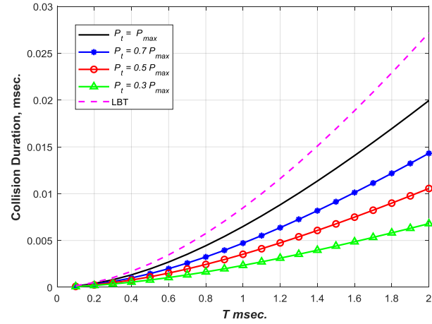
Figure B.14.2: collision duration vs. SUs' frame time, for different levels of SUs' power.
