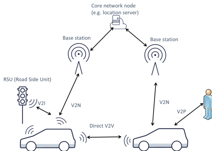
Figure 3.5-1 Various V2X communication scenarios
