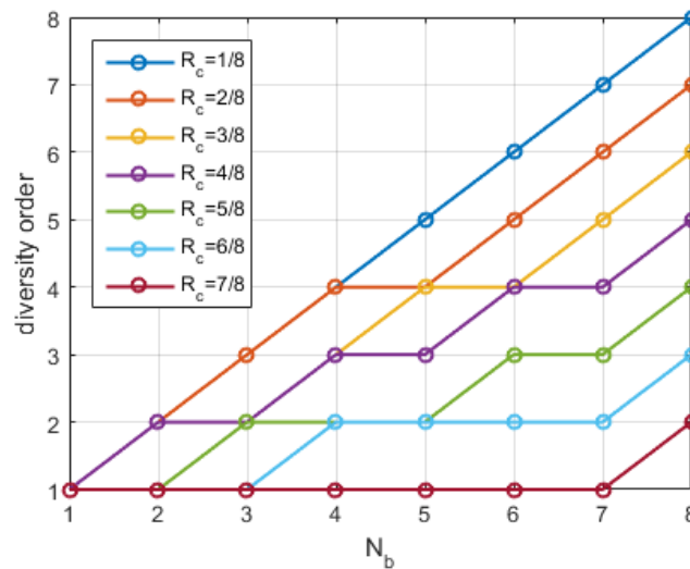
Figure B.7.1 Maximum diversity order for code rate R_c and N_b fading blocks
