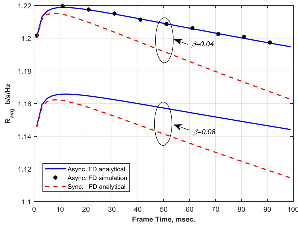
Figure B.14.3: normalized throughput for synchronous and asynchronous transmission vs. secondary's frame duration.
