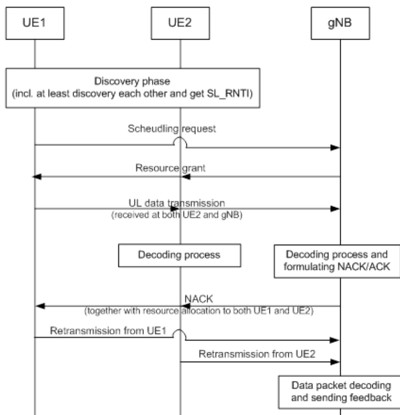
Figure 3.3-6 Example procedure for sidelink assisted reliable communication
