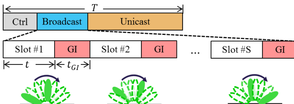
Figure 3.2-1 Illustration of frame structure.
