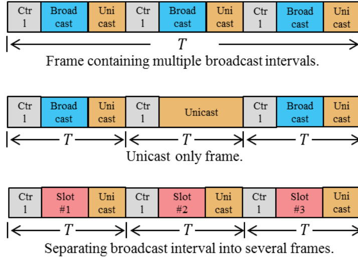
Figure 3.2-2: Illustration of different frame structure designs.
