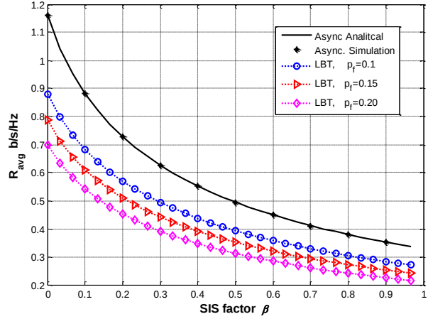
Figure B.14.4 variation of D2D throughput against different self-interference suppression capability of OBUs.
