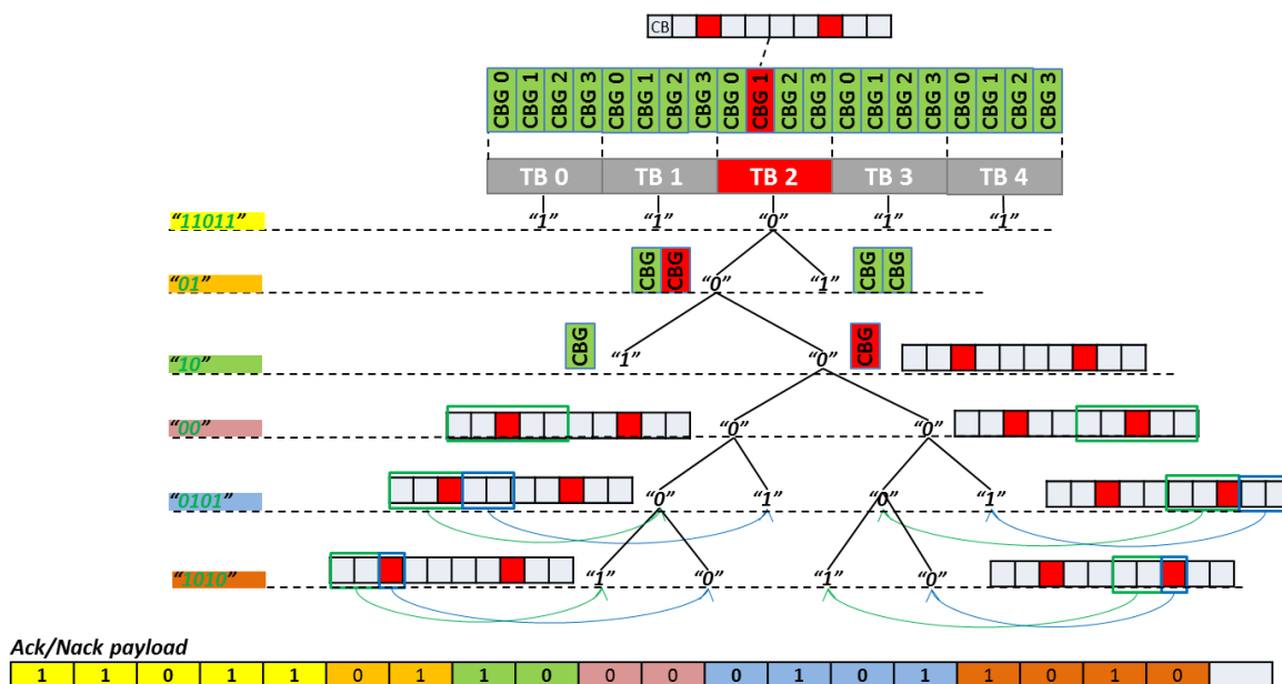
Figure B.3.5: Example of proposed binary search based HARQ-ACK feedback for multiple TBs.
