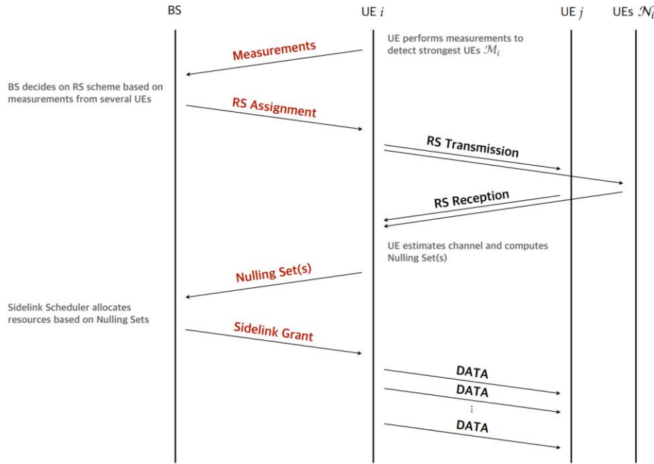
Figure B.11-1: Message sequence chart of proposed procedure
