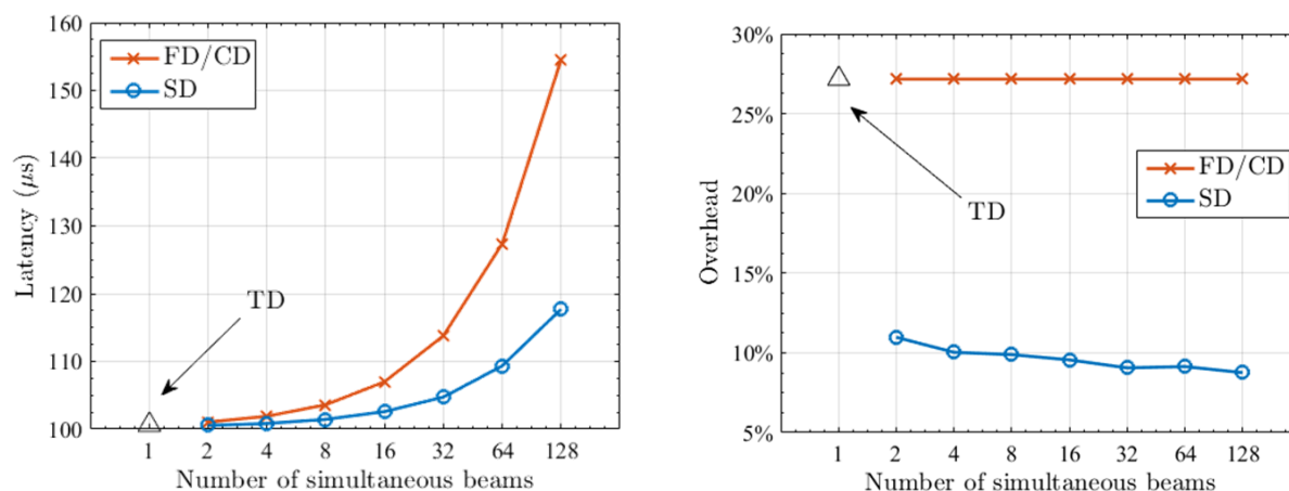
Figure B.6.1: Performance of different broadcast schemes for V2X applications are compared in terms of (a) latency and (b) overhead.
