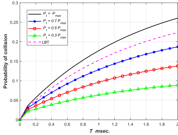
Figure B.14.1: Probability of collision of D2D users with cellular users vs. SUs' frame time, for different levels of SUs' power.
