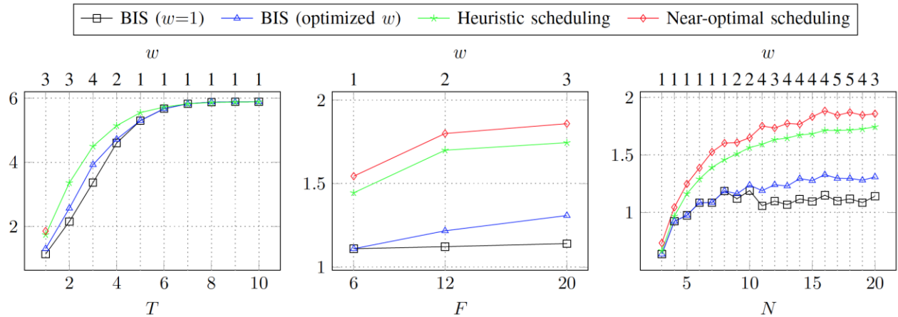
Figure B.10.2 Average number of successful links per V-UE for various scheduling algorithms.
