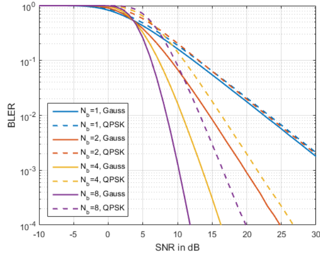
Figure B.7.2 BLER performance in finite lengths (128 resource elements) for R=1.6 bits/use
