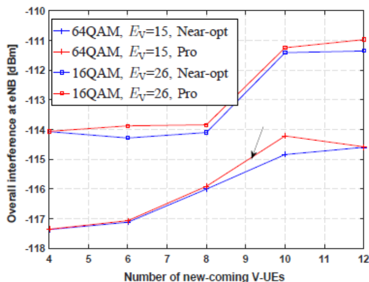
Figure B.13.1 Overall interference at the BS, with one TTI message transmission. Here new-coming V-UEs denote the V-UEs whose messages transmission starts from the current time.
