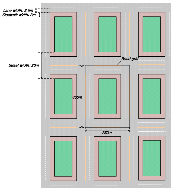
Figure A.1.4.1: Road configuration for urban traffic efficiency and safety evaluation [3GPP-36885]
