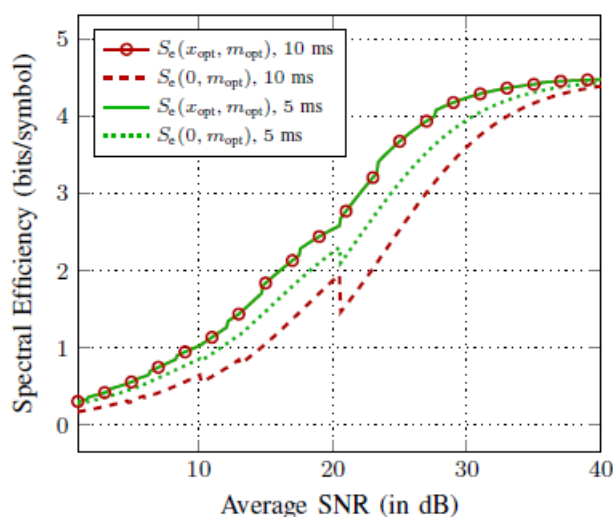
Figure B.9.2: Optimal Spectral Efficiency S_e(x_{opt}, m_{opt}) and spectral efficiency S_e(0, m_{opt}) vs Average SNR for different latency budgets, with reliability 1 \cdot 10^{-4} .
