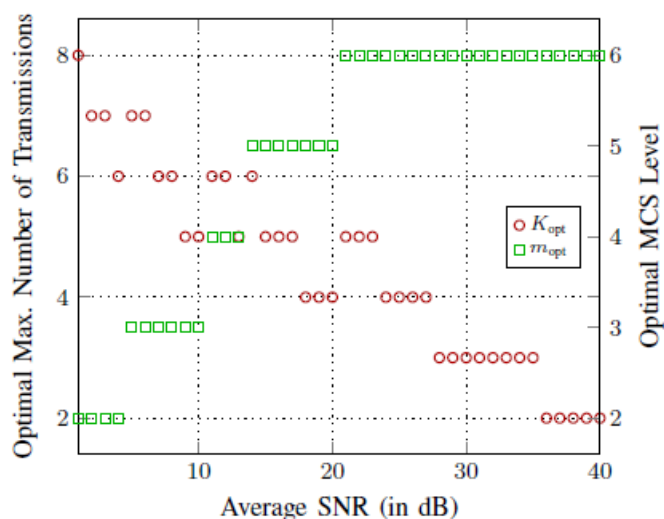
Figure B.9.1: Optimal Max Number of Transmissions and Optimal MCS Level vs Average SNR, with latency budget 5 ms and reliability 1 \cdot 10^{-4} .
