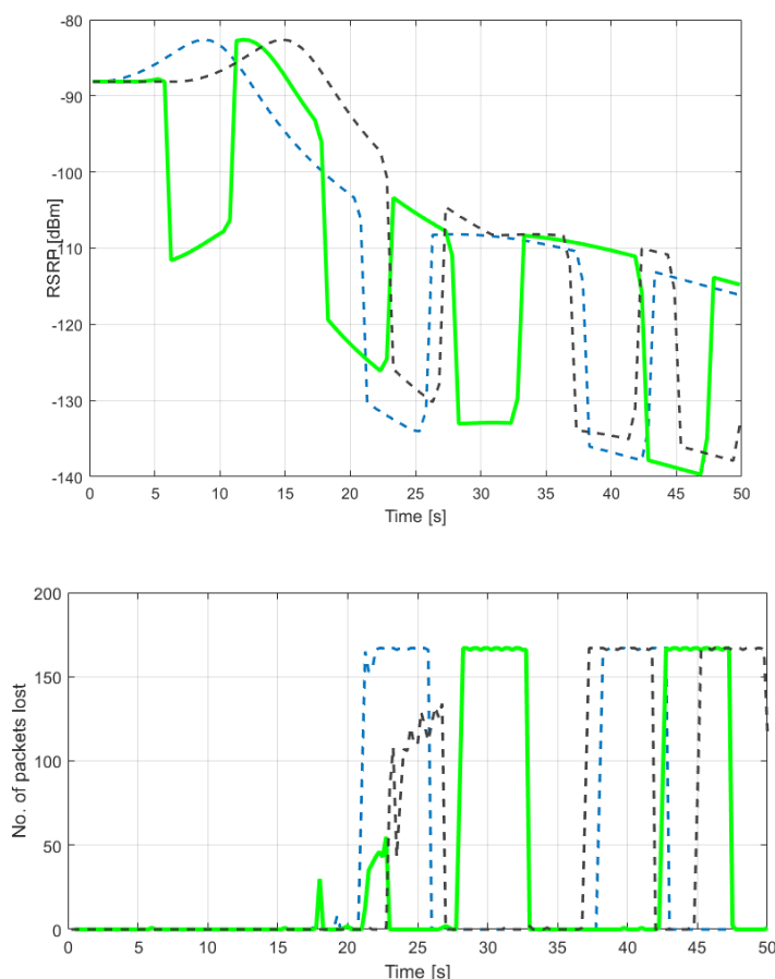
Figure B.5.1 Received average power (RSRP) vs. time for 3 cars forming a cluster (top) and corresponding packet losses measured (bottom). Conditions of each car are represented by individually coloured curves.
