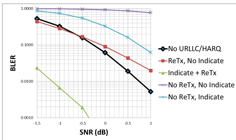
Figure B.3.2: Preemption effect on robustly coded transmission with/without HARQ and indication on preemption at Rx.
