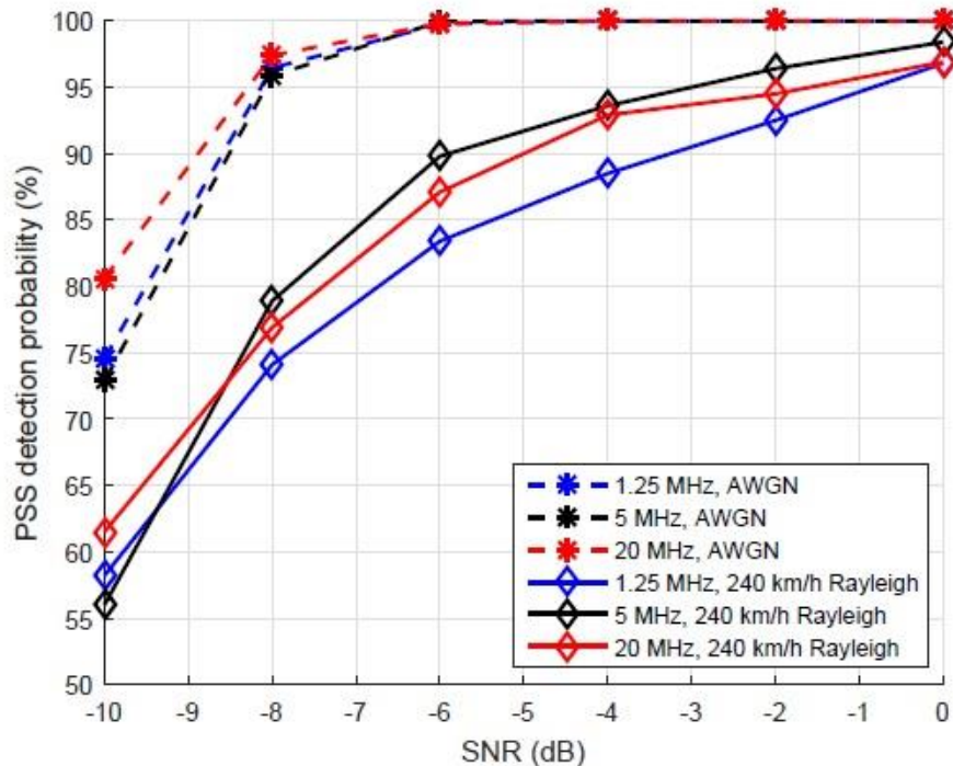
Figure 3.3-5– Probability of correct sequence detection over the SNR.
