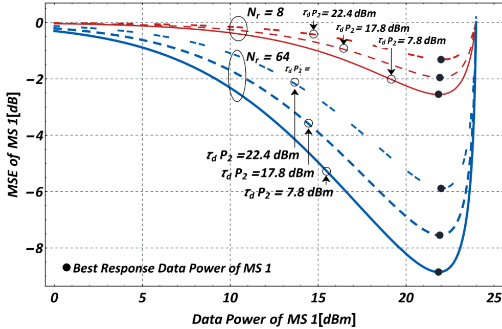
Figure B.4.1: The MSE of User-1 in a two-player pilot-to-data power ratio tuning game. Increasing the number of receive antennas from N_r=8 to N_r=64 and tuning the pilot-to-data power ratio under a total power constraint (24 dBm) helps to reduce the MSE. ( \tau_d denotes the number of pilot symbols, and \tau_d P_2 denotes the total pilot power used by MS2.)
