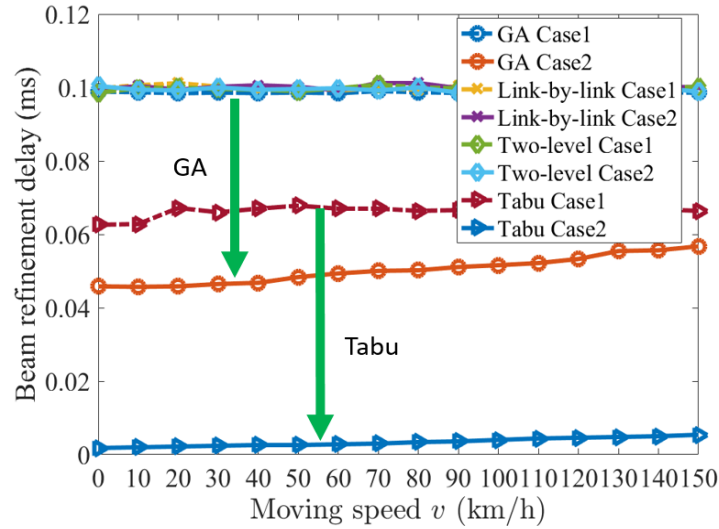
Figure B.2.1: The beam refinement delay for a broad range of user speeds with the considered methods. The green arrows refer to the reduction from Case 1 to Case 2 for the GA and the Tabu search.
