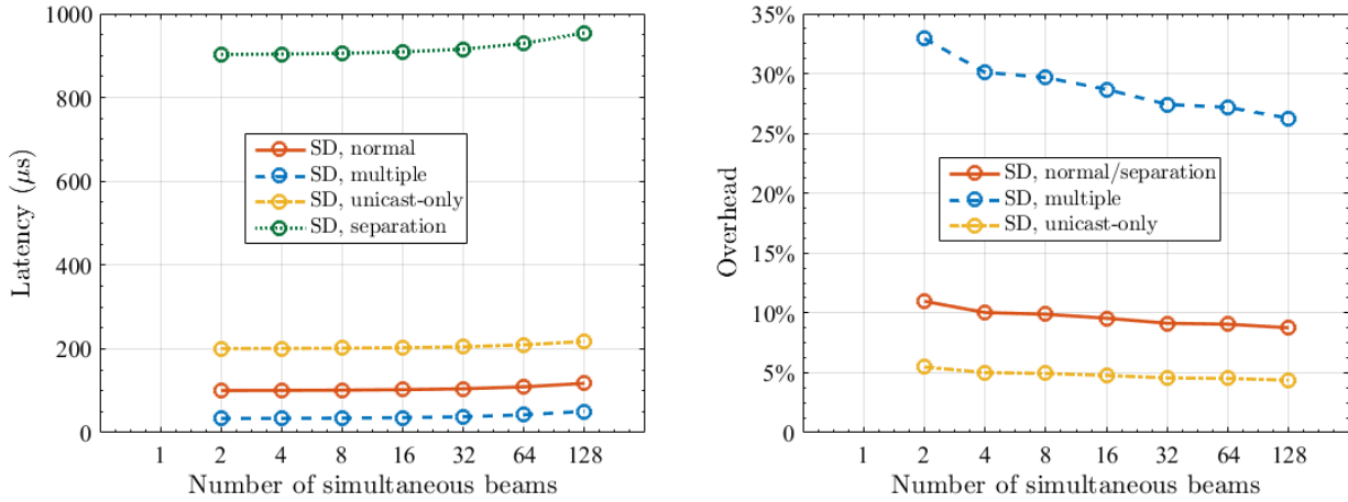
Figure B.6.1: Performance of different broadcast schemes for V2X applications are compared in terms of (a) latency and (b) overhead.
