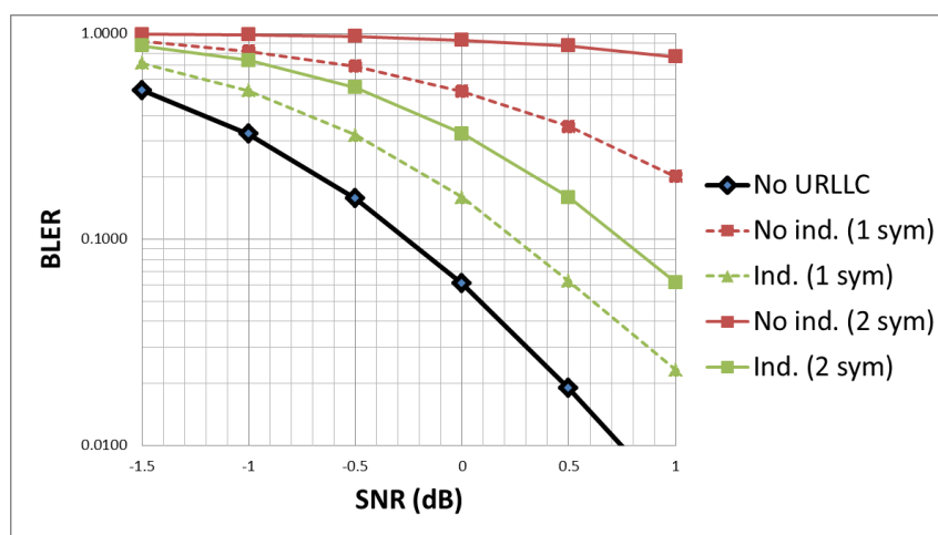
Figure B.3.1: Preemption effect on robustly coded transmission with/without indication on preemption at Rx. Simulation assumptions: QPSK for both eMBB, URLLC; 11 bytes TB size; 1/3 TBCC coding; Interleaving within CB; 1-2 symbols for URLLC; 14 symbols for eMBB; 12 SCs of 15kHz SCS; 1 Tx-1 Rx; ideal channel estimation; soft HARQ combining at UE.
