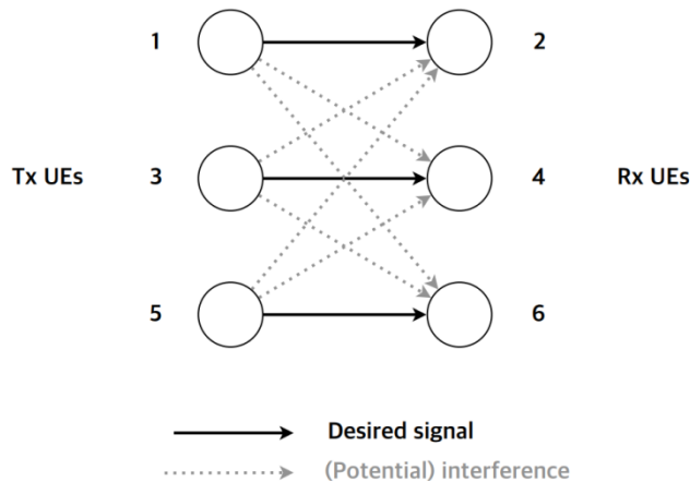
Figure B.11.2: Example with 3 antennas per vehicle – receiving UEs use fixed rank-one receive filters.
