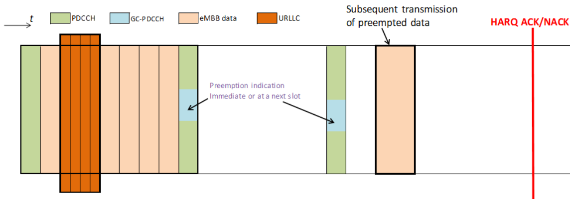
Figure B.3.6: Subsequent transmission of preempted data.
