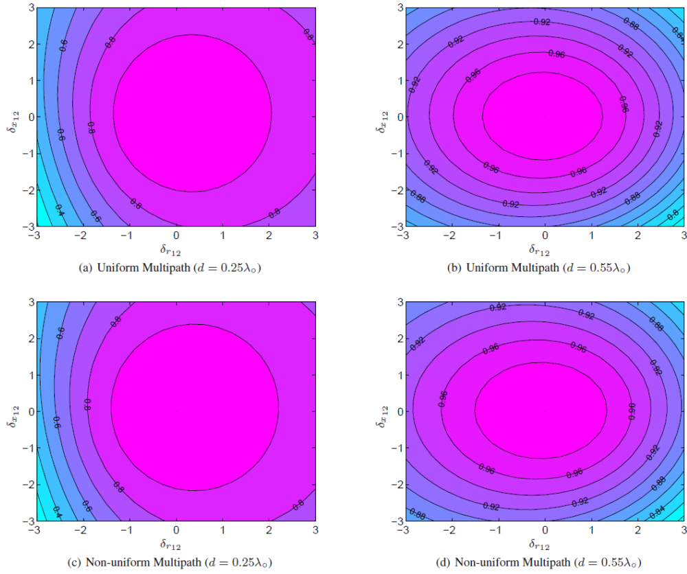
Figure B.1.3: Dependency of open-circuit decoupling method on Z-matrix.
