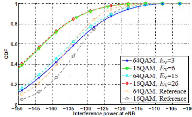
Figure B.13.2. Except from the CDF of the measured interference power per RB at the BS
