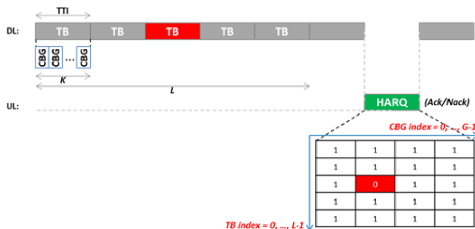
Figure B.3.4: Example for conventional HARQ-ACK feedback on multiple TBs
