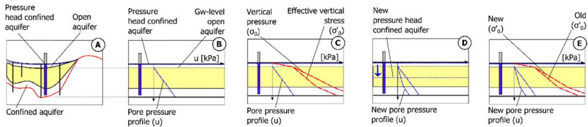
Fig. 3. One simulation sequence of pore pressure (B), effective vertical stress (C), new pressure head due to groundwater drawdown in confined aquifer (D), and new effective stress (E).
