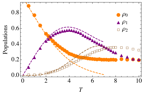
FIG. 3. (Color online) Vacuum (filled orange circles), single-photon (filled purple triangles) and two-photon (open brown squares) populations for the reconstructed state of the output field for a drive strength \Omega^* and as a function of T . Here we set \gamma = 1 as the unit. The dashed lines of the same colors correspond to the analytical solutions of these populations which we include for comparison.
