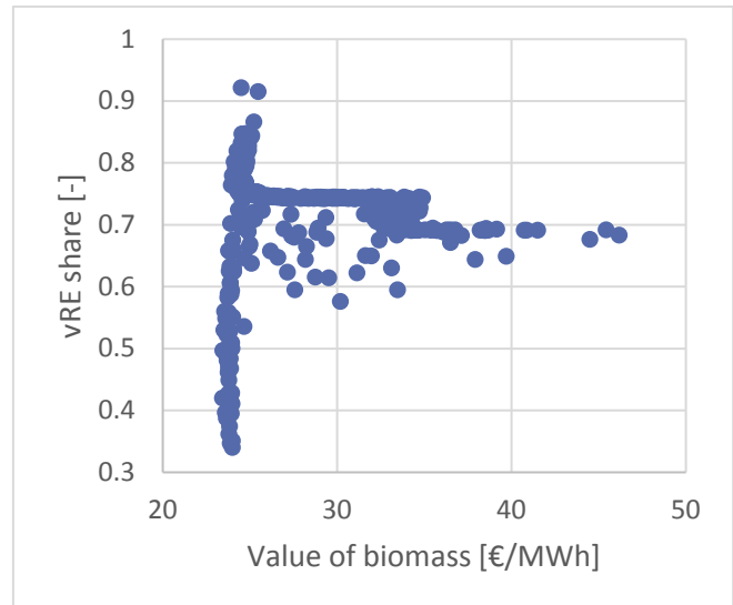
Fig. B.2. The vRE share is plotted against the biomass value for the base case in ES3 with 20% biomass availability.
