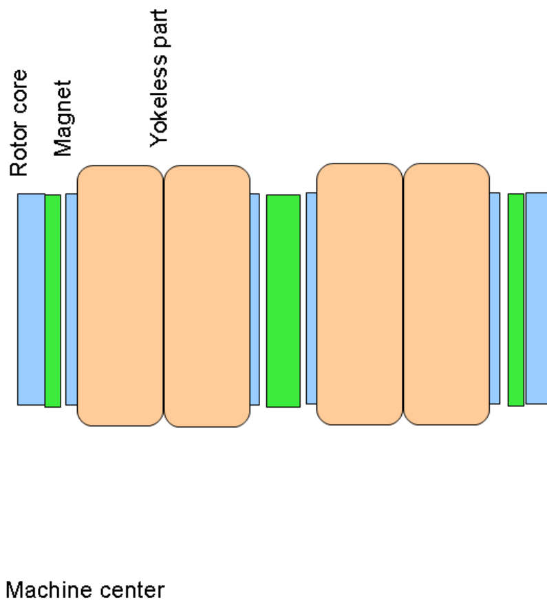
Figure 5. Two section of the yoke-less axial flux machine.
