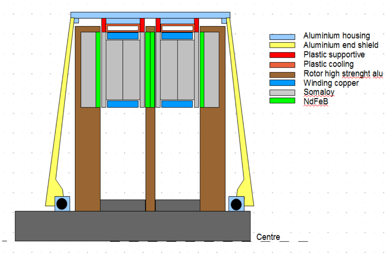
Figure 15. Axial flux machine. Three rotor discs and two yokeless stators
