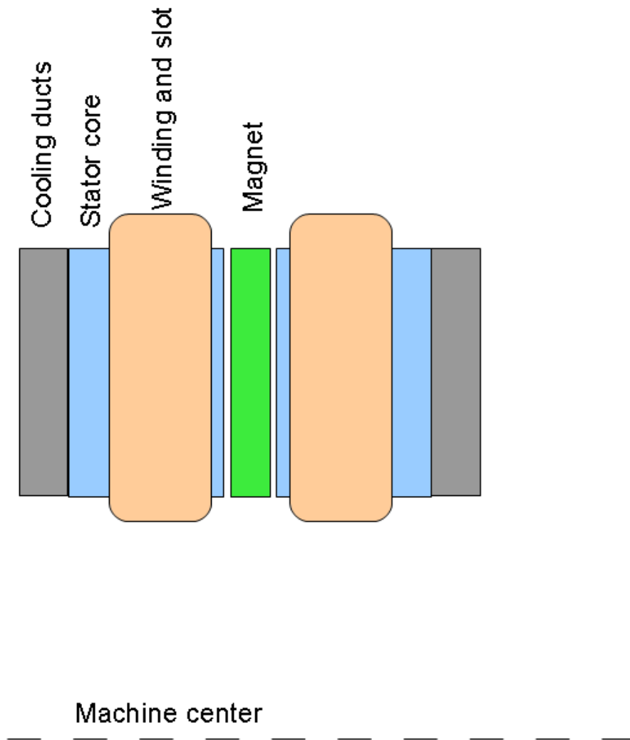
Figure 3. Axial flux machine arrangement cross section
