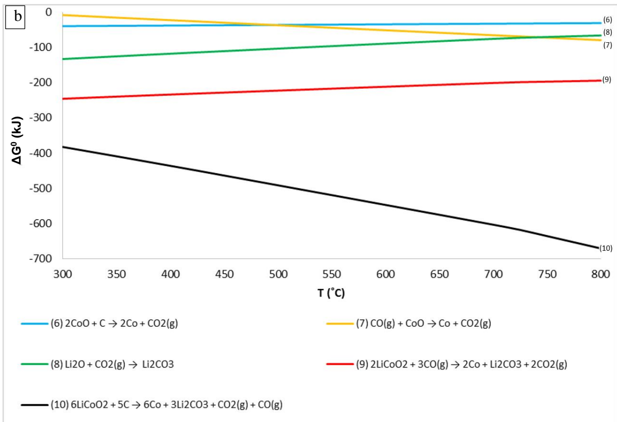
Figure 11a and b : Plots of \Delta G^0 (kJ) vs T (°C) for the reduction of \text{LiCoO}_2 and by-products with C or CO.
