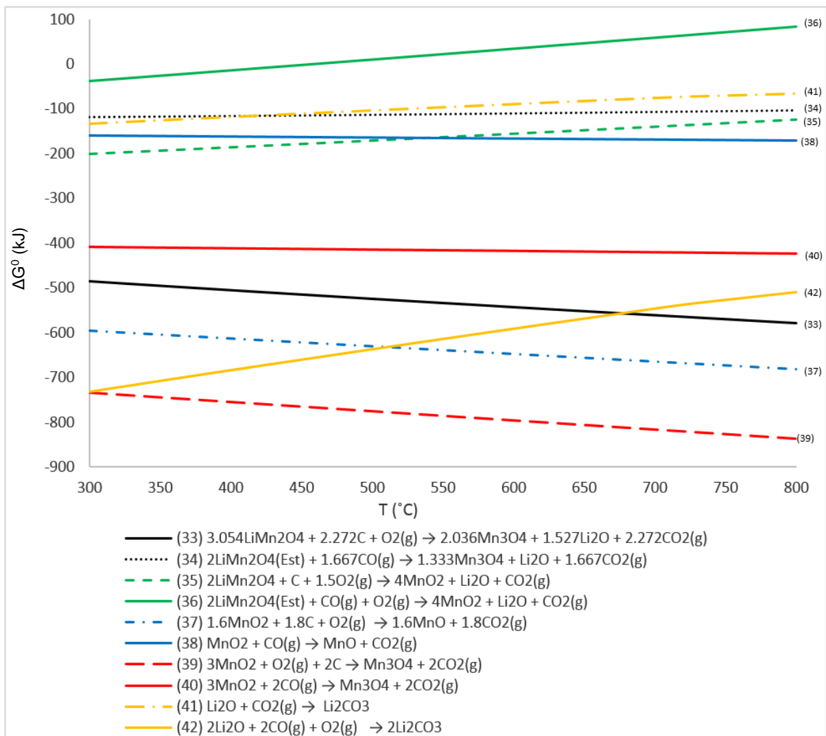
Figure 16: Plot of \Delta G^0 (kJ) vs T ( ^{\circ}\text{C} ) for the reduction of \text{LiMn}_2\text{O}_4 .
