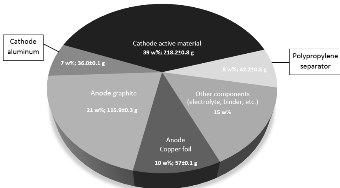
Figure 7: Mass balance of used material.
