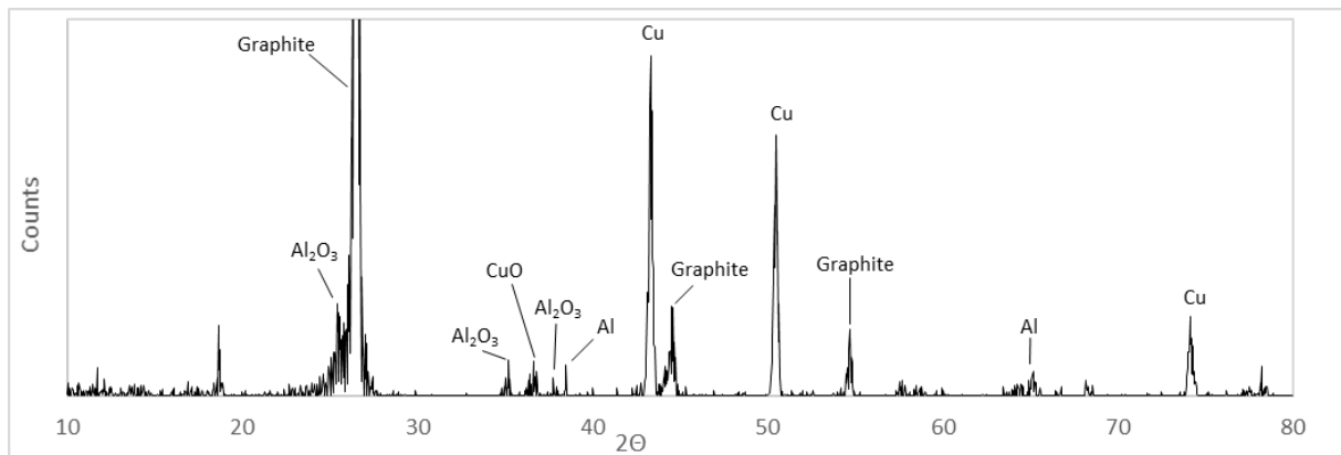
Figure 9: The XRD diffractogram of mixed electrode materials (anode and cathode).
