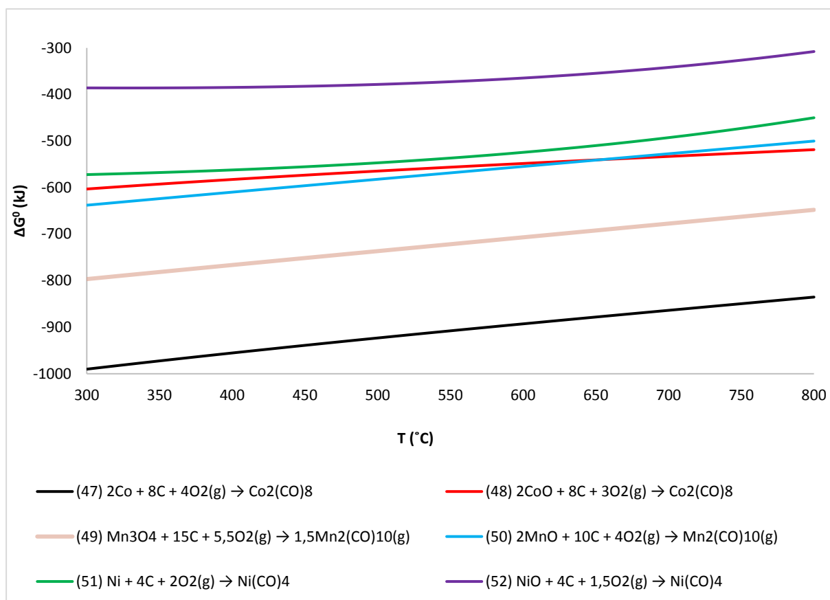
Figure 17: Plot of \Delta G^\circ (kJ) vs T ( ^\circ\text{C} ) for the reaction of formation of metal carbonyls,
