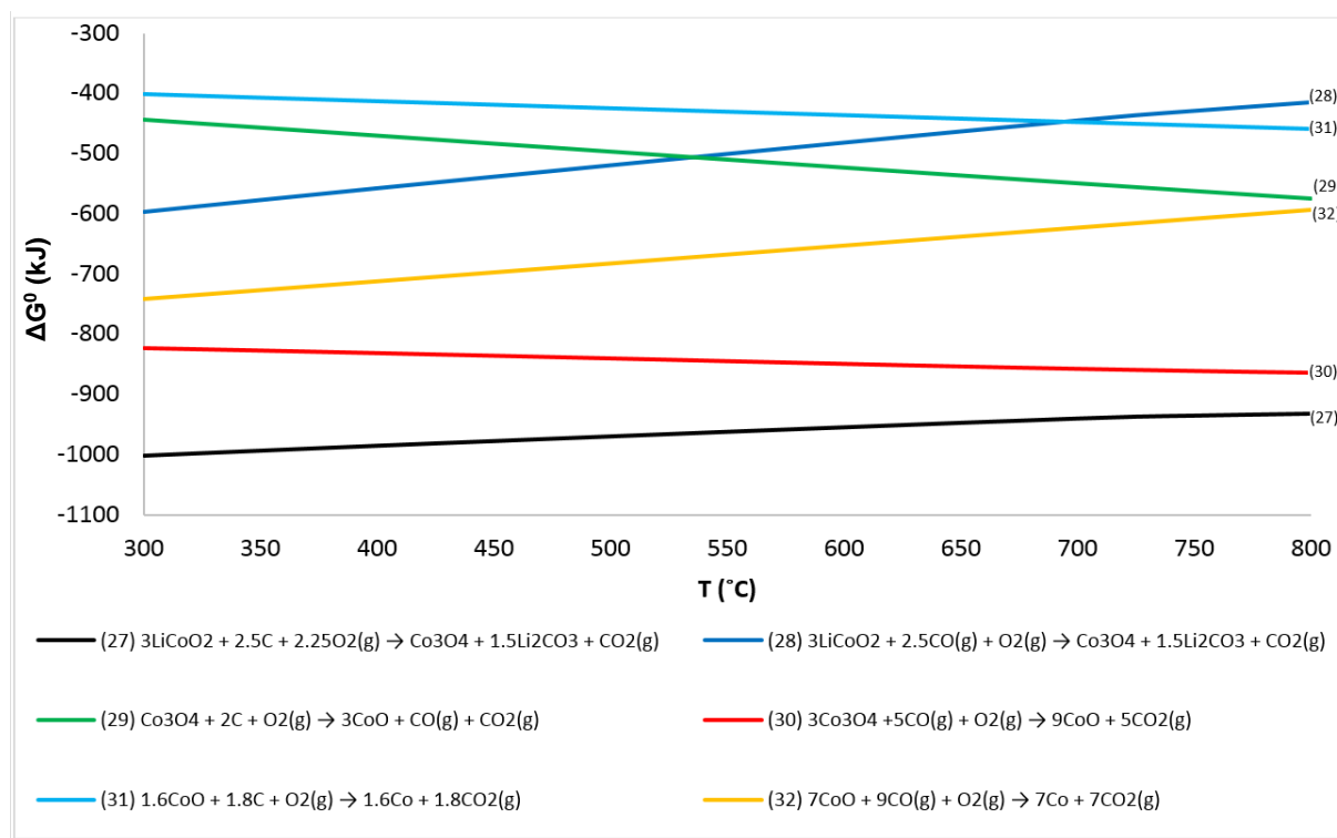
Figure 15: Plot of \Delta G^0 (kJ) vs T ( ^{\circ}\text{C} ) for the reduction of \text{LiCoO}_2 with \text{C} .
