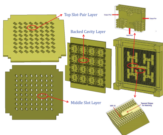
Fig. 1. Configuration of the proposed corporate-feed slot array antenna based on groove gap waveguide.
