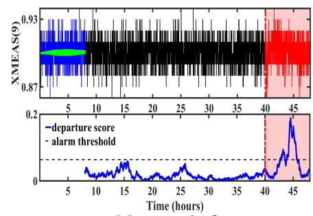
Figure 5: Stealthy attack \mathcal{SA3} compromising the sensor variable xMEAS(10) detected in sensor variable xMEAS(9) .
