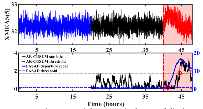
Figure 9: Both PASAD and the AR method successfully detect the direct damage attack \mathcal{DA}2 .
