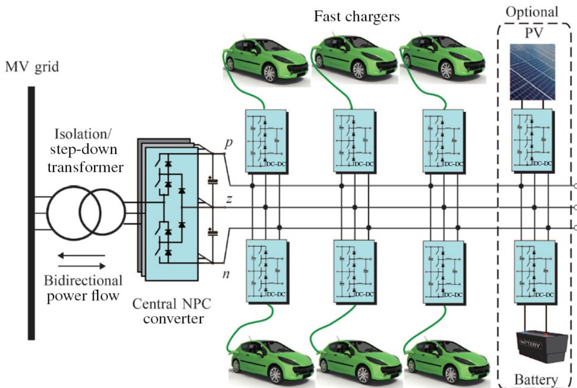
Figure 11. Central DC-link
