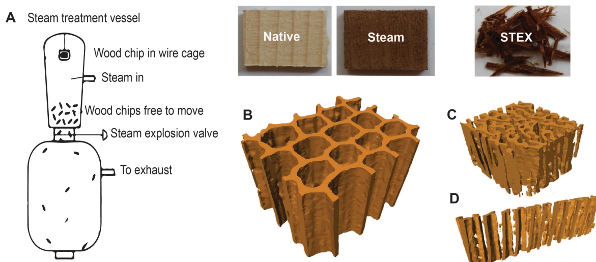
Figure 11. Simplified illustration of the STEX equipment used for steam treatment or STEX-treatment of wood chips ( Paper I ) (A). Wood samples and X-ray tomography images of the internal structures of intact wood (native or steam-treated) (B) or STEX-treated and structurally deformed wood with the formation of microcracks in the cell walls (C-D). (Figures courtesy of Muhammad Muzamal.)
