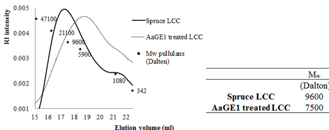
Figure 19. RI detector response from SEC analysis of spruce LCC, before (solid line) and after (dotted line) GE hydrolysis. The peak shifts towards lower molecular weight (M w ) (higher elution volume), which indicates the release of lignin from carbohydrates as a result of GE action. The table gives the molecular weight of the LCC fraction before and after GE treatment.
