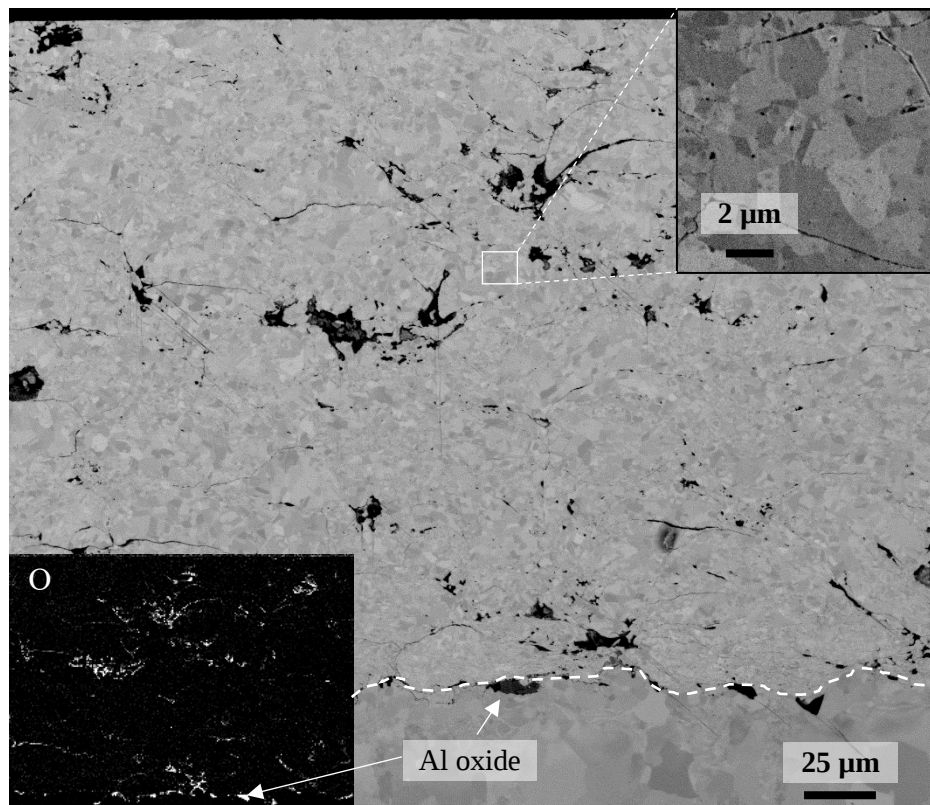
Figure 40: SEM image using BSE of a cross section of a NiCr-coated sample after exposure in 5% O 2 + 20% H 2 O + N 2 at 600 °C for 168 hours. The signal for oxygen from the EDX analysis is located at the bottom left of the picture. A higher magnification of an area of the coating is shown at the top right. The dashed line represents the coating/substrate interface.
