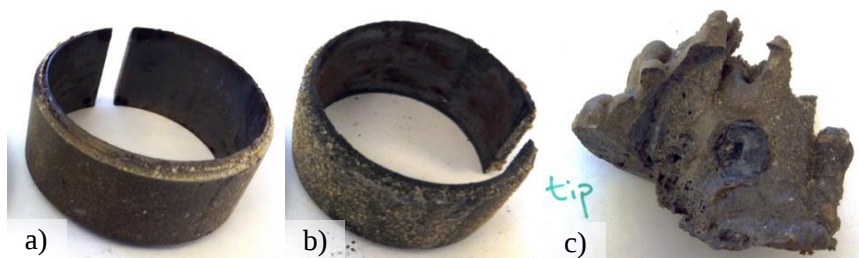
Figure 50: Photographs of three different amounts of deposits accumulated on Sanicro 28 for three different settings after 2-hour exposures. A) small amount, b) moderate amount, and c) large amount.
