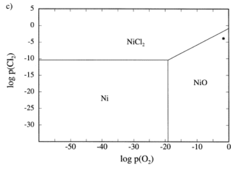
Figure 7: Thermodynamic stability diagrams of the systems Fe-O 2 -Cl 2 (a), Cr-O 2 -Cl 2 (b) and Ni-O 2 -Cl 2 (c) at 600 °C [44].
