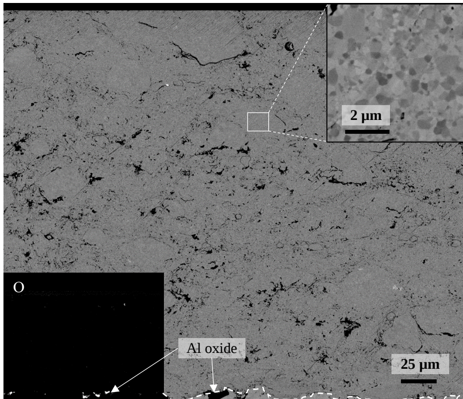
Figure 43: SEM image using BSE of a cross section of a NiCrAlY-coated sample in 5% O 2 + 20% H 2 O + N 2 at 600 °C for 168 hours. The signal for oxygen from the EDX analysis is located at the bottom left of the picture. A higher magnification of an area is shown at the top right. The dashed line represents the coating/substrate interface.
