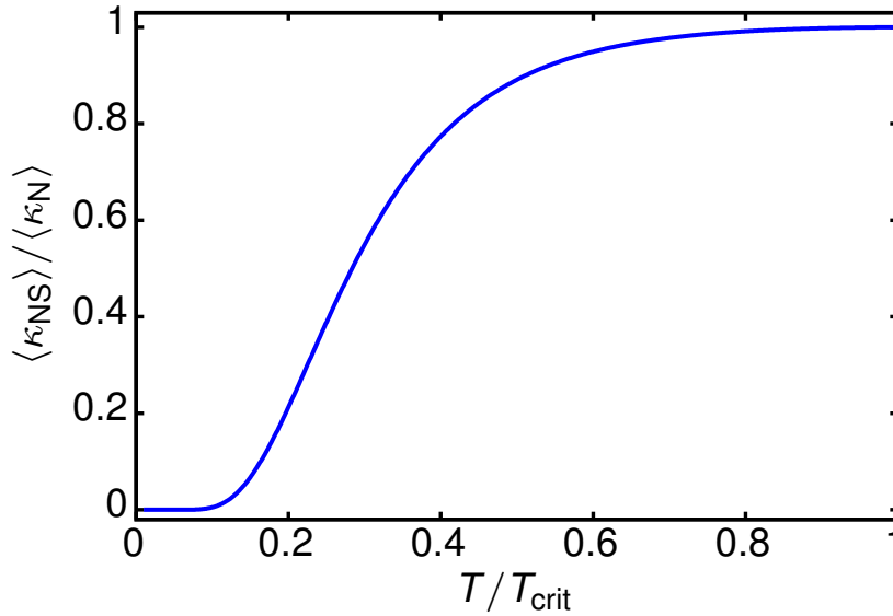
Figure 4.3: Temperature dependent of the average heat conductance of NS junction normalized to the average of normal heat conductance.
