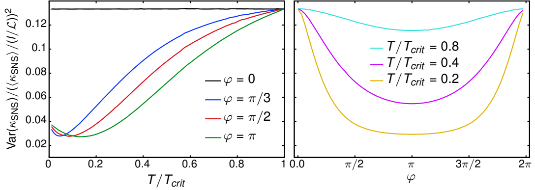
Figure 3.7: Temperature- and phase-dependence of the heat conductance fluctuations \text{Var}[\kappa_{\text{SNS}}] / (\langle \kappa_{\text{SNS}} \rangle / (l/L))^2 . (Left) \text{Var}[\kappa_{\text{SNS}}] / (\langle \kappa_{\text{SNS}} \rangle / (l/L))^2 as function of T for different \varphi . The black line at 2/15 represents the normalconducting result, see Eq. (3.18a). (Right) \text{Var}[\kappa_{\text{SNS}}] / (\langle \kappa_{\text{SNS}} \rangle / (l/L))^2 as function of \varphi for different T s.
