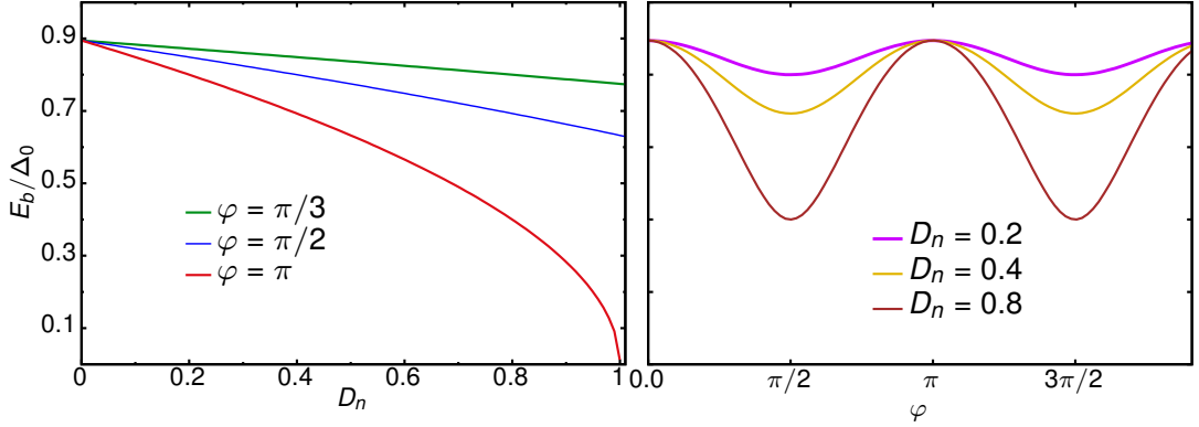
Figure 3.3: Phase and transmission dependence of the Andreev bound state energy. The temperature is T/T_{\text{crit}} = 0.2 and \Delta_0 is the superconducting energy gap at zero temperature.
