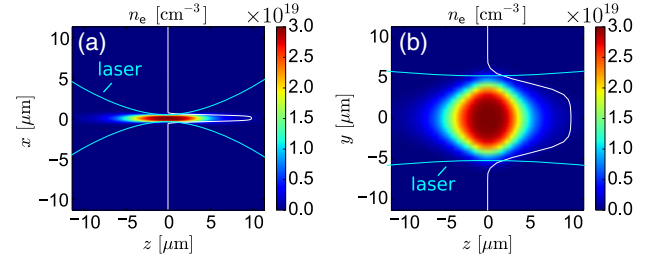
Fig. 7. Electron density in the (a) zx and (b) yz planes after ionization of an argon gas with initial neutral density n_a = 3 \times 10^{19} \text{ cm}^{-3} ( \approx 1 \text{ bar} ) by a 2C elliptically shaped laser pulse ( E_\omega = 40 \text{ GV/m} , E_{2\omega} = 20 \text{ GV/m} , t_0 = 50 \text{ fs} , w_{0,x} = \lambda_{\text{FH}} = 0.8 \mu\text{m} , w_{0,y} = 8 \mu\text{m} ). The respective electron density profiles at focus ( z = 0 ) are visualized by the bright white lines. The waist of the focused laser is tracked by the light blue lines.
