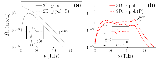
Fig. 8. Angularly integrated far-field spectra for the elliptical beams from Fig. 7 (solid lines) and corresponding results from 2D simulations assuming translational invariance in y (dashed lines). The insets show the forward-emitted THz pulses recorded at z = 12.7 \mu\text{m} behind the plasma.
