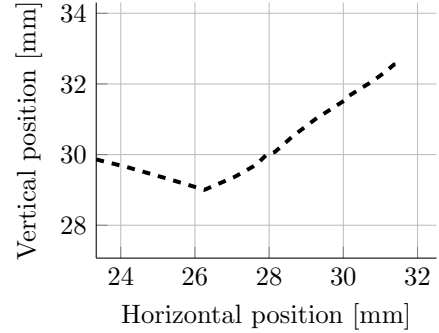
(d) Prediction of fatigue crack growth directions and comparison to experiment.
