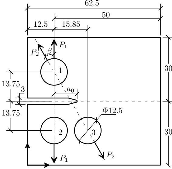
Figure 3.4: Setting of the CTS experiment in [67].
