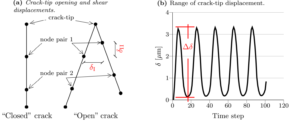
Figure 2.7: Definitions of crack-tip displacements and range of crack-tip displacement.
