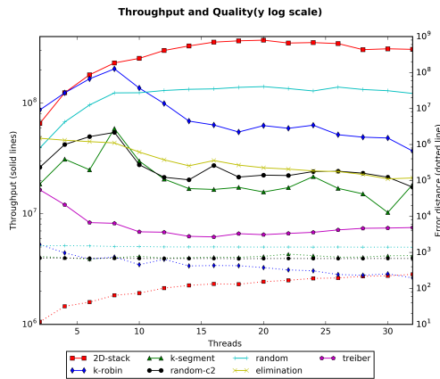
Figure 2: Throughput and observed accuracy as concurrency increases.
