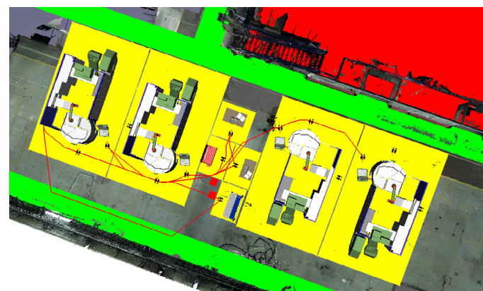
Fig. 15. The rotation algorithm creates a layout with a collision-free walking route based the initial solution. Courtesy by GKN.
