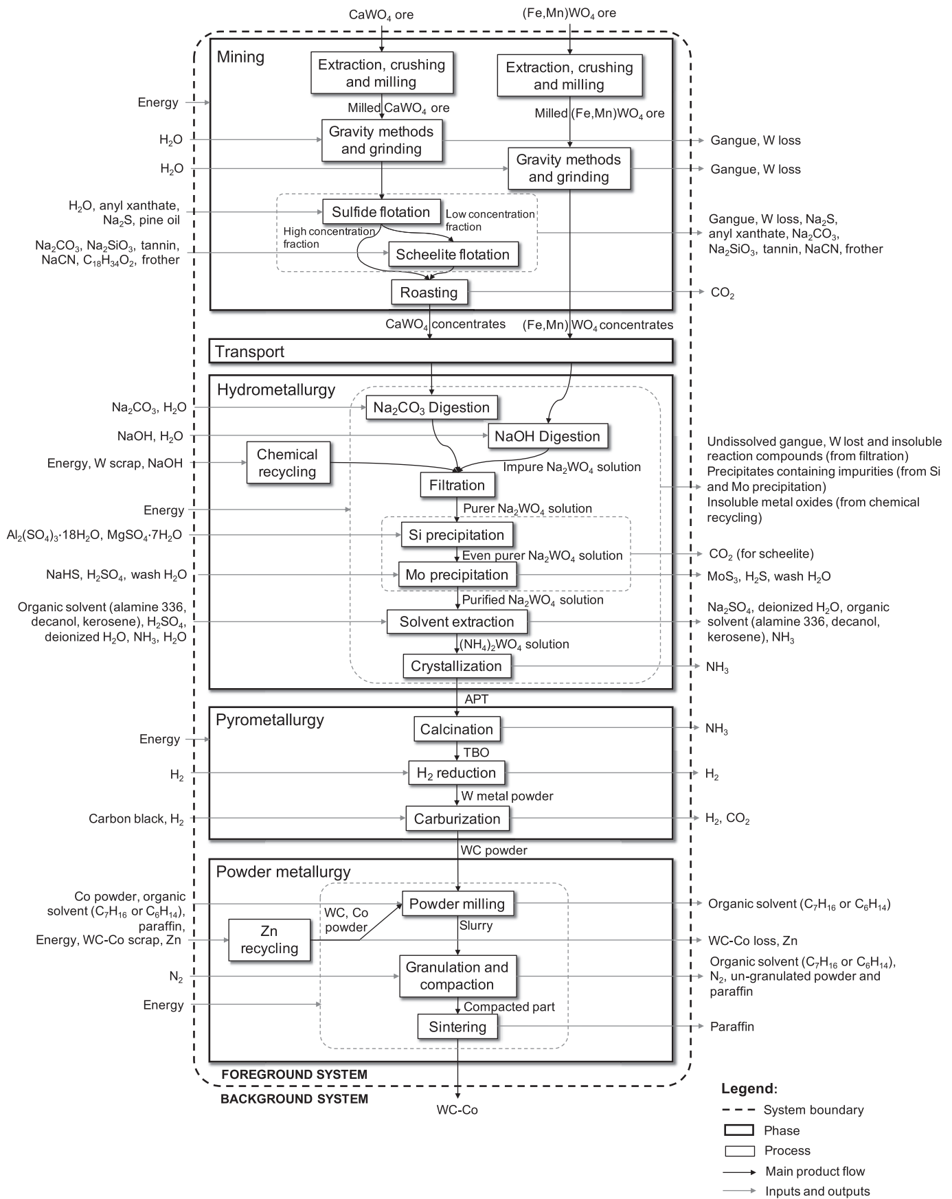
Fig. 1. Flowchart for the typical non-Chinese tungsten carbide with cobalt (WC-Co) production. \text{CaWO}_4 = scheelite, (\text{Fe,Mn})\text{WO}_4 = wolframite, \text{H}_2\text{O} = water, W = tungsten, \text{Na}_2\text{S} = sodium sulfide, \text{Na}_2\text{CO}_3 = sodium carbonate or soda ash, \text{Na}_2\text{SiO}_3 = sodium silicate, \text{NaCN} = sodium cyanide, \text{C}_{18}\text{H}_{34}\text{O}_2 = oleic acid, \text{CO}_2 = carbon dioxide, \text{NaOH} = sodium hydroxide, \text{Na}_2\text{WO}_4 = sodium tungstate, \text{Al}_2(\text{SO}_4)_3 \cdot 18\text{H}_2\text{O} = aluminum sulfate solution, \text{MgSO}_4 \cdot 7\text{H}_2\text{O} = magnesium sulfate solution, Si = silica, Mo = molybdenum, \text{NaHS} = sodium hydrosulfide, \text{H}_2\text{SO}_4 = sulfuric acid, \text{MoS}_3 = molybdenum trisulfide, \text{H}_2\text{S} = hydrogen sulfide, \text{NH}_3 = ammonia, \text{Na}_2\text{SO}_4 = sodium sulfate, (\text{NH}_4)_2\text{WO}_4 = ammonium tungstate, ammonium paratungstate (APT), tungsten blue oxide (TBO), \text{H}_2 = hydrogen, WC = tungsten carbide, Co = cobalt, \text{C}_7\text{H}_{16} = heptane, \text{C}_6\text{H}_{14} = hexane, Zn = zinc and \text{N}_2 = nitrogen.
