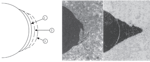
(a) Sketch. (b) Experimental observation.
