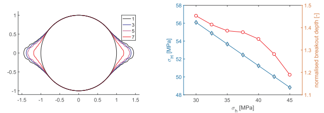
(a) Breakout shape. (b) Stress states.
