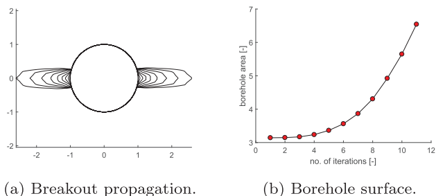
Fig. 13. Compaction induced breakouts.
