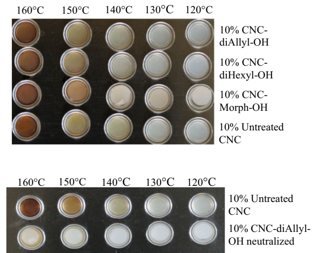
Figure 3 Upper photograph: visual appearance of the composites containing 10 wt% CNC after exposure for 8 min to (from right to left) 120, 130, 140, 150 and 160 °C. Lower photograph: visual appearance of the composites containing 10 wt% untreated CNC and 10 wt% CNC-diAllyl-OH from the pH-neutralised system after exposure for 8 min to (from right to left) 120, 130, 140, 150 and 160 °C.
