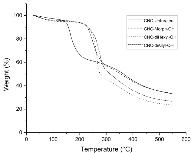
Figure 2 Thermogravimetric curves showing the thermal degradation of untreated and surface-modified CNC.
