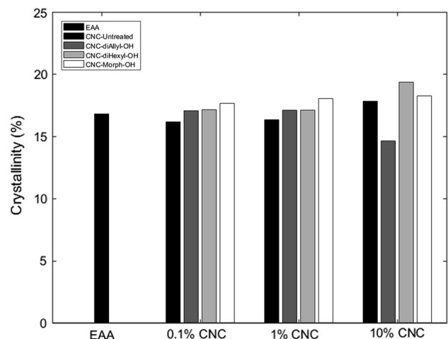
Figure 12 Total crystallinity of the unfilled EAA and the CNC-containing composites.
