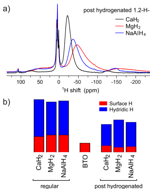
Figure 13. (a) 1 H MAS NMR spectra of posthydrogenated samples. (b) Comparison of relative strengths and shift contributions to the 1 H MAS NMR signal integral for regular and posthydrogenated 1.2-H samples.
