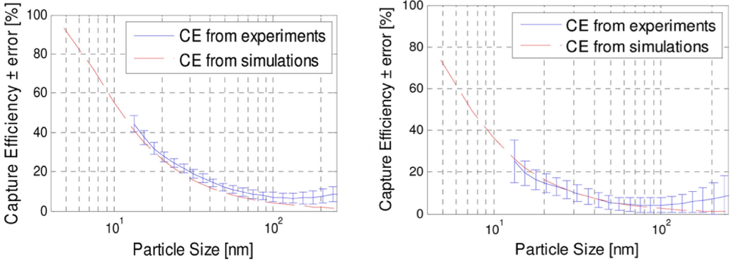
Figure 2.3: Deposition efficiency of NaCl nanoparticles in a bare cordierite substrate at Re = 7.8 (left) and Re = 24 (right) at 150\text{ deg C} . The error bars represent confidence intervals. Note the similarities between experiments and simulations.
