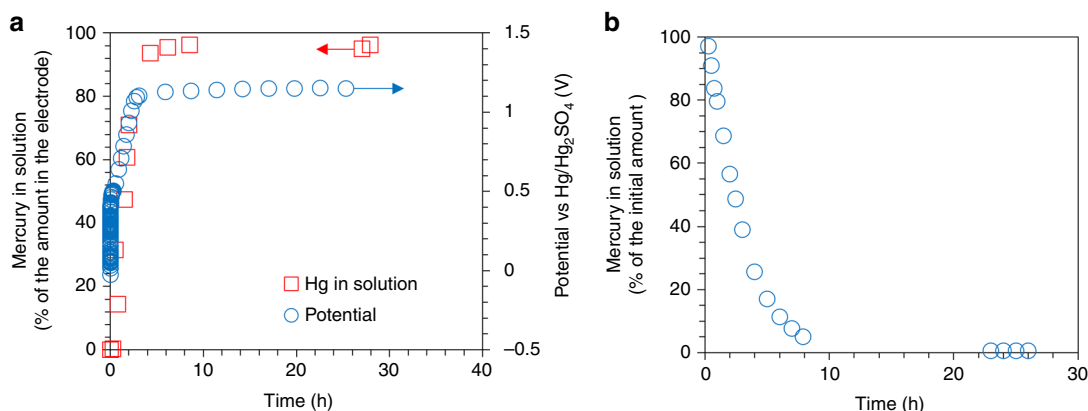
Fig. 5 Regeneration of nano-film electrodes and the use of large surface area electrodes. a The increase of mercury concentration in pure 1 mol L -1 nitric acid solution upon applying a 40 \mu A current to a 100 nm platinum electrode previously used for mercury retrieval (red squares, left axis), and the recorded potential (blue circles, right axis). Counter electrode: platinum wire. Reference electrode: Hg/Hg 2 SO 4 . b Retrieval of mercury from 50 mL 1 mol L -1 nitric acid solution containing 10 mg L -1 mercury. Working electrode: 50%wt. platinum nanoparticles on carbon black, deposited on carbon paper support. Counter: platinum wire. Reference: Hg/Hg 2 SO 4 . Working potential = 0.16 V vs. RHE
