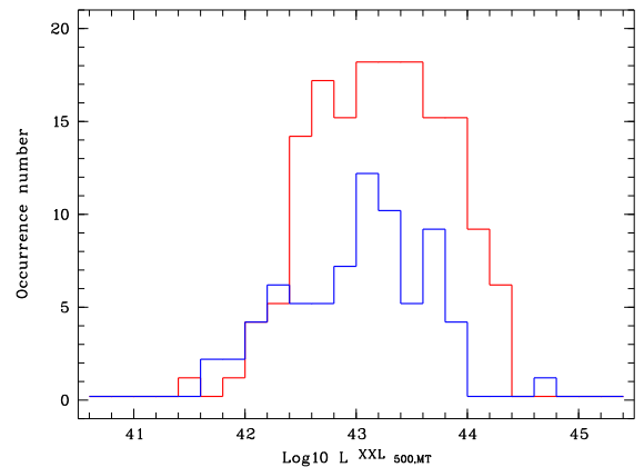
Fig. 7. X-ray luminosity ( L_{500, \text{MT}}^{\text{XXL}} in log unit of \text{erg s}^{-1} in the [0.5–2] keV band) distribution of clusters having a spectroscopic redshift and a luminosity determination. Red histogram: the C1 sample; blue histogram: the C2 sample.
