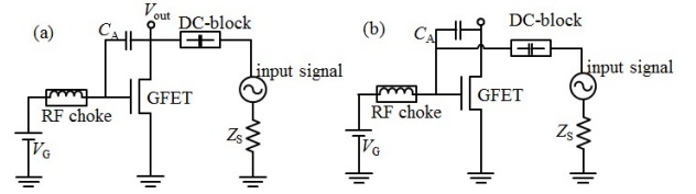
Fig. 2. Two possible topologies of GFET detector with (a) v_{\text{gs}} = v_{\text{in}} \cos(\omega t) and v_{\text{ds}} = \alpha v_{\text{in}} \cos(\omega t + \theta) , (b) v_{\text{ds}} = v_{\text{in}} \cos(\omega t) and v_{\text{gs}} = \alpha v_{\text{in}} \cos(\omega t + \theta) .
