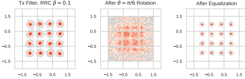
Fig. 3.3. Effect of dynamic equalization. (a) Transmitted signal shaped with a root-raised cosine filter with \beta = 0.1 . (b) resulting constellation after a small polarization rotation. (c) Constellation after dynamic equalization.
