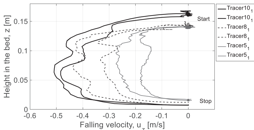
Figure 1. Maximum and minimum measured falling velocity, u_z , over bed height, z , for three different tracers, Tracer 10, 8, and 5, after 10 repetitions.
