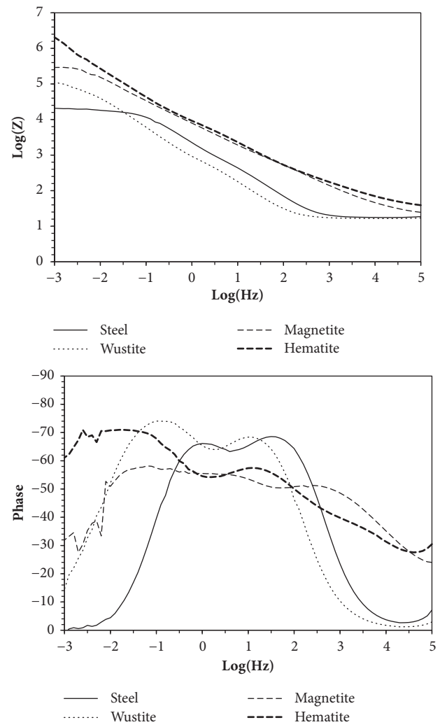
FIGURE 4: Example of Bode plots obtained in sat. Calcium hydroxide solution with 0.6 M Cl - .
