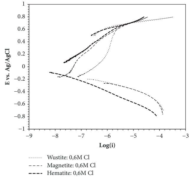
FIGURE 8: Anodic and cathodic potentiodynamic potential curves for the iron oxides exposed in saturated \text{Ca}(\text{OH})_2 solution with 0.6 \text{ M Cl}^- .
