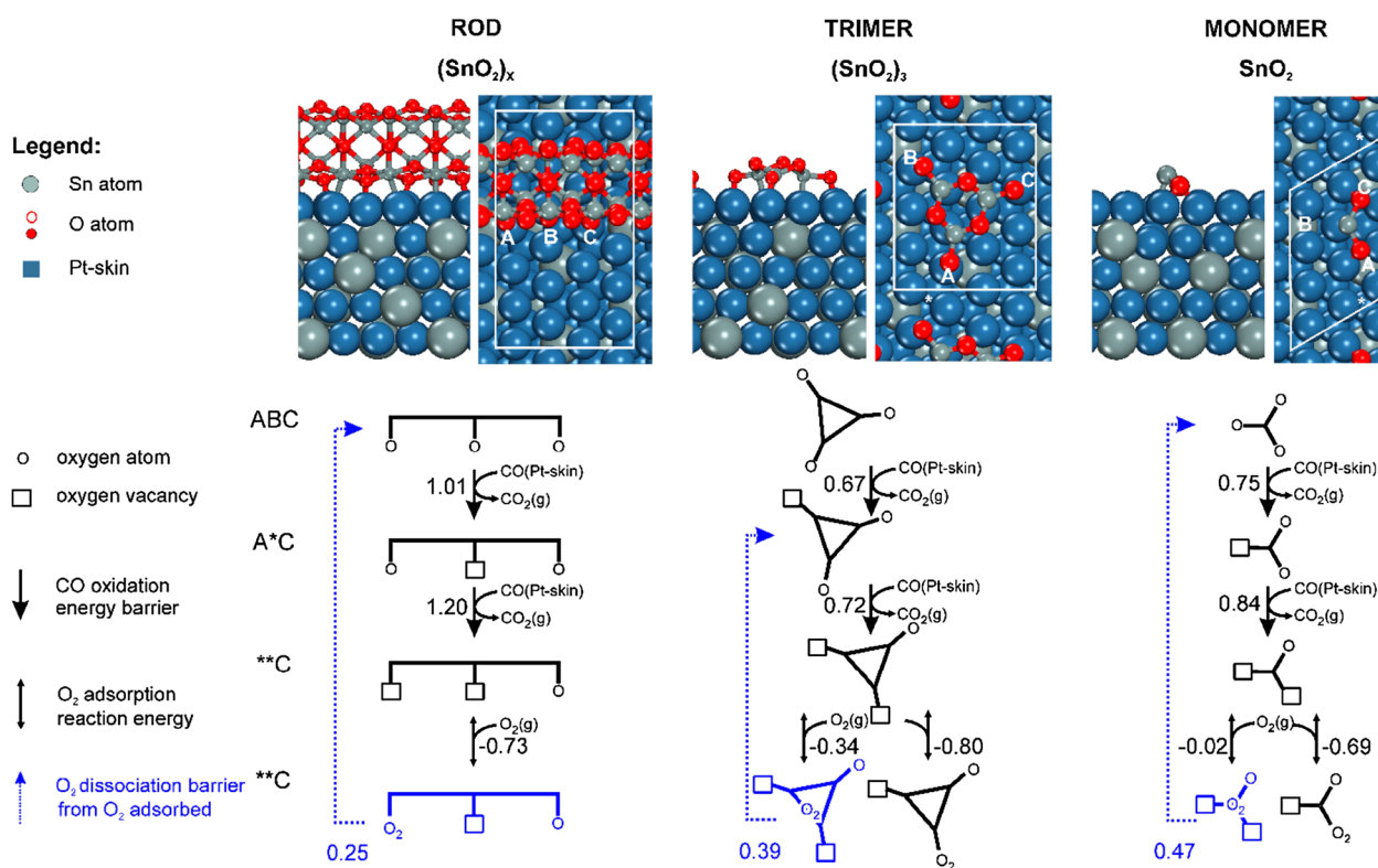
Fig. 4 Schematic representation of putative catalytic cycles of CO oxidation for the considered systems. The \text{O}_2 dissociation barriers are here given with respect to adsorbed \text{O}_2
