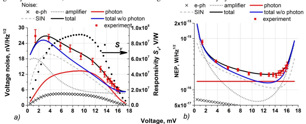
Fig. 6. Various components of voltage noise (a) and NEP (b) versus bolometer voltage. Curves - theory, red markers - experiment. Photon temperature 330 mK, absorbed power 20 pW. Photon noise dominates over CEB noise from 11 to 14 mV.
