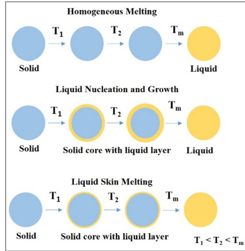
Figure 14: Different melting hypotheses for nanoparticles (Redrawn from [36]).
