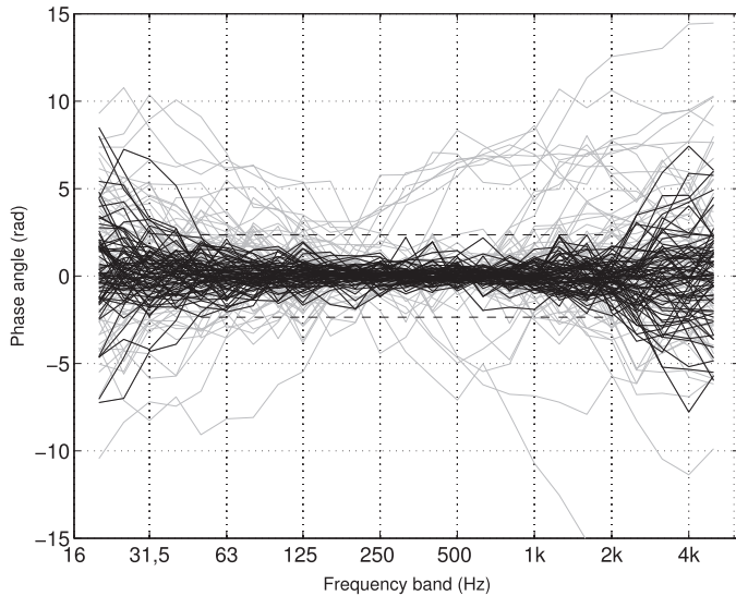
Fig. 4. Phase angles over frequency bands for all sound clips at location 4. The dashed black lines show the coherency limits, the black lines are the recordings that are assessed to be coherent, and the grey lines the recordings that are not coherent.
