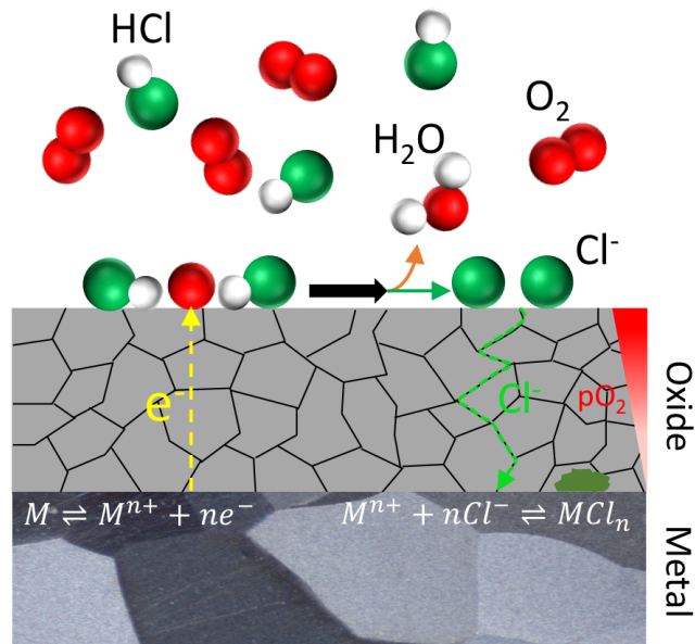
Figure 16: Schematic illustration of the chlorine-induced corrosion mechanism using the electrochemical approach.
