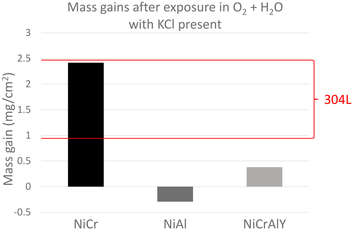
Figure 45: Mass gains of coated samples after exposure for 168 hours in 5% O 2 + 20% H 2 O + N 2 at 600 °C with KCl present. The red lines display the mass gain range (based on measured oxide thickness) for a bulk 304L sample exposed to the same conditions.
