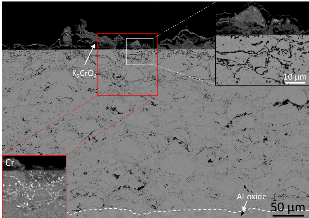
Figure 48: SEM-BSE cross section image of NiCrAlY coating after exposure in 5% O 2 + 20% H 2 O + N 2 at 600 °C with KCl present for 168 hours. The box in the bottom left corner shows the EDX-map for Cr. The dashed line indicates the coating/substrate interface. Remaining Al-oxide from grit blasting of substrate observed at coating/substrate interface.
