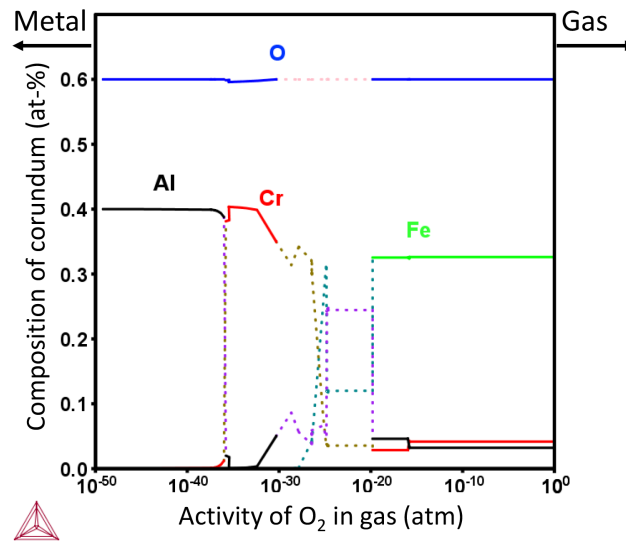
Figure 33: Thermodynamic calculation of the composition of corundum against different activities of O 2 in gas for FeCrAl 2 Si performed by Dr Sedigheh Bigdeli using ThermoCalc. The dotted lines show pO 2 regions where corundum is metastable.
