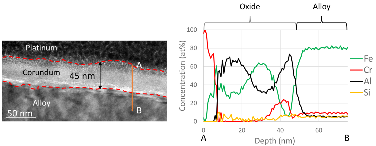
Figure 32: STEM cross section image of the thin protective oxide on FeCrAl 2 Si (left) with EDS-data (right) after exposure in O 2 + N 2 at 600 °C for 168 hours. TEM analysis performed by Dr Vijayshankar Asokan.
