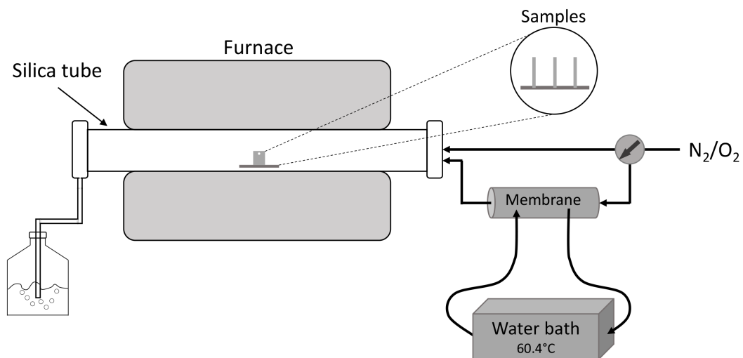
Figure 18: Schematic illustration of the tube furnace set-up used in this study.
