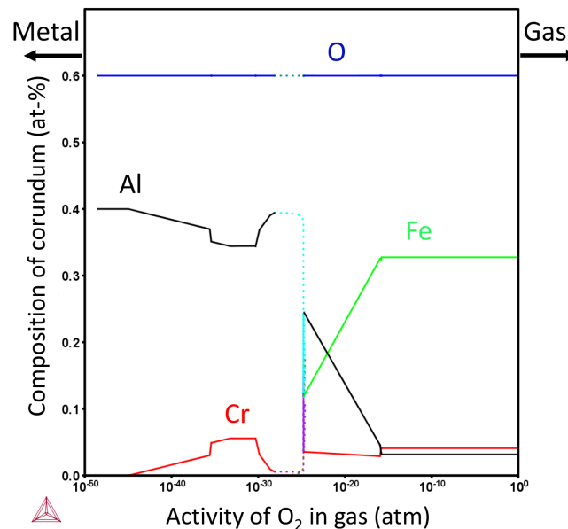
Figure 31: Thermodynamic calculation of the composition of corundum against different activities of O 2 in gas for FeCrAlO 3 Si performed by Dr Sedigheh Bigdeli using ThermoCalc. The dotted lines show a pO 2 region where corundum is metastable.
