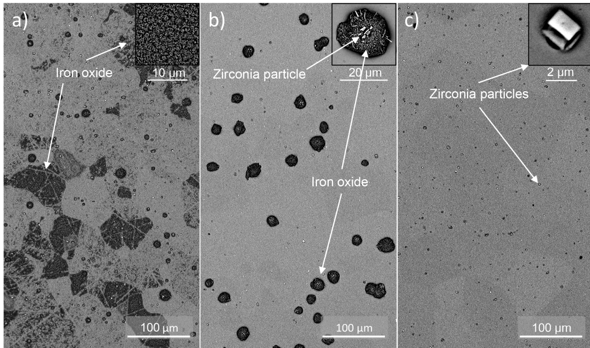
Figure 28: SEM-BSE plan view images of a) FeCrAl0Si, b) FeCrAl1Si and c) FeCrAl2Si after exposure in 5% O 2 + N 2 (bal.) for 168 hours at 600 °C.
