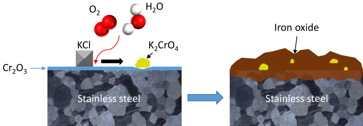
Figure 14: Schematic illustration of the breakdown of the chromium oxide due to formation of \text{K}_2\text{CrO}_4 in the presence of KCl.
