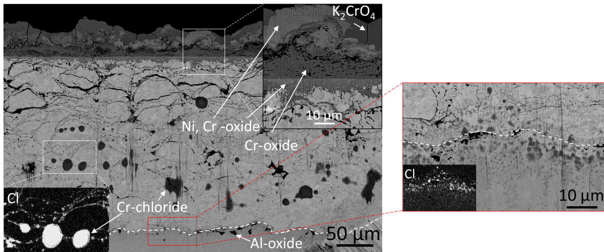
Figure 46: SEM-BSE cross section image of NiCr coating after exposure in 5% O_2 + 20% H_2O + N_2 at 600 °C with KCl present for 168 hours. The dashed line shows the coating/substrate interface. Remaining Al-oxide from grit blasting of substrate observed at coating/substrate interface.
