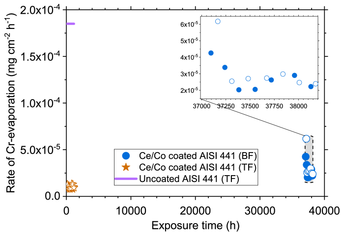
Figure 4.6: Rate of Cr-evaporation as a function of time for AISI 441 exposed up to 38 100 h at 800 °C. Samples were exposed either in box furnaces (BF) by AB Sandvik Materials Technology or in tube furnaces (TF) at Chalmers. The Cr-evaporation measurements were all conducted in tube furnaces.
