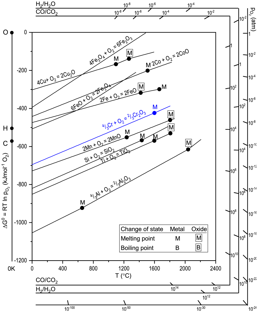
Figure 2.2: Elingham Diagram for selected oxides based on [43, 45].
