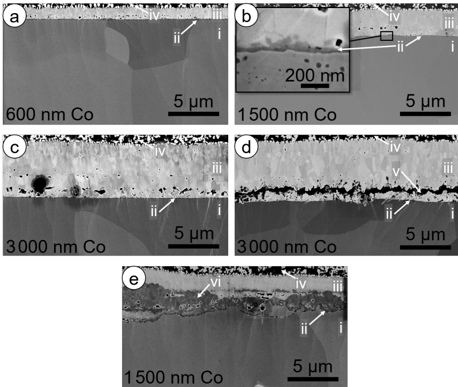
Figure 4.1: SEM micrograph of cross sections of Co-coated Crofer 22 APU exposed for 500 h at 600 °C. All samples were Co-coated according to the following specifications: a) pre-oxidized sample with 600 nm Co coating, b) pre-oxidized sample with 1500 nm Co coating, c) pre-oxidized sample with 3000 nm Co coating, d) pre-oxidized sample with 3000 nm Co coating, which showed signs of spallation after exposure, and e) non-pre-oxidized sample with 1500 nm Co coating. The phases are identified as follows: i) substrate alloy, ii) \text{Cr}_2\text{O}_3 , iii) \text{Co}_3\text{O}_4 , iv) Pt electrode, v) spallation crack, and vi) (\text{Co,Cr,Fe})_3\text{O}_4 .
